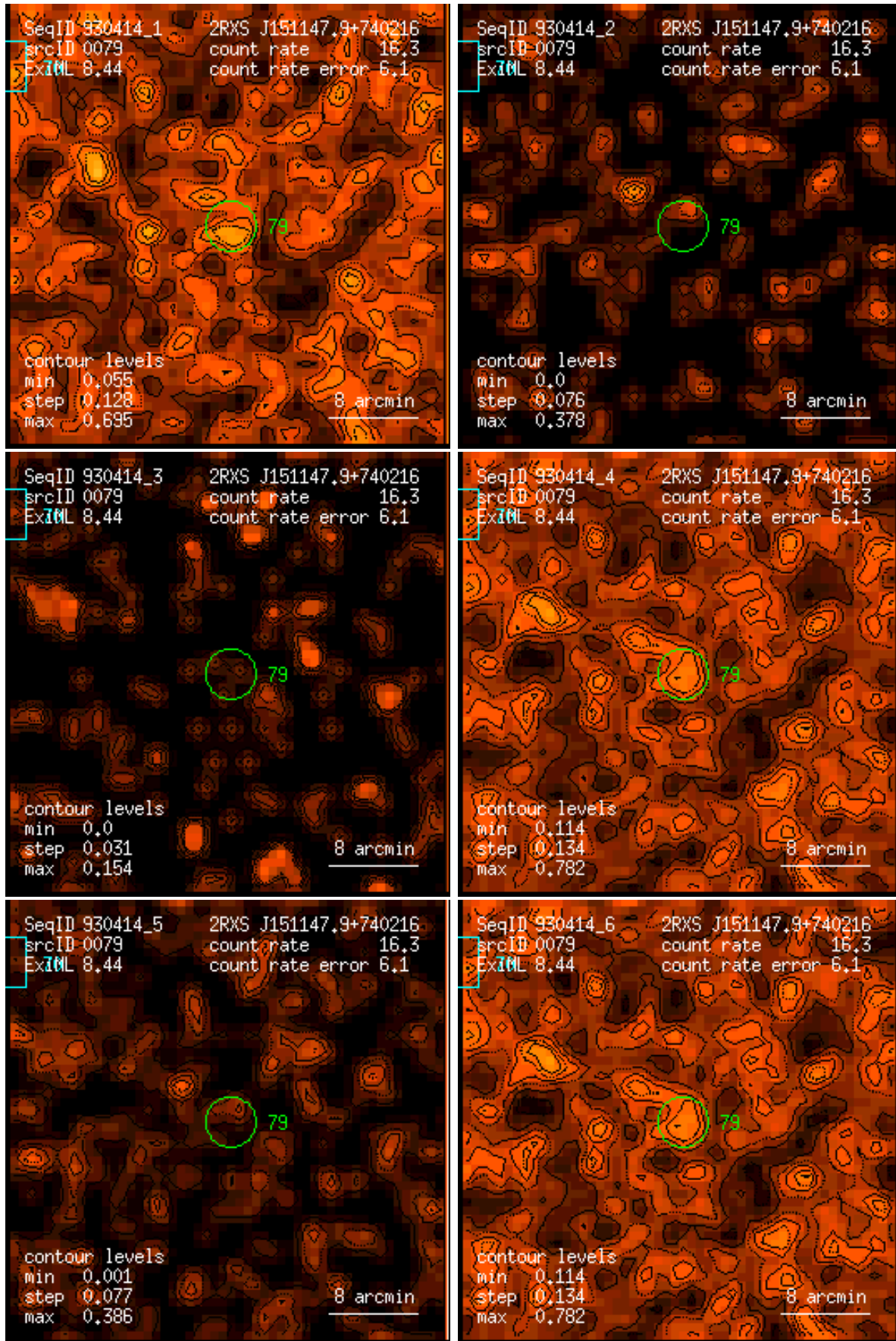
Figure 79: RASS 930414: detection 0079: band rate images, Gaussian filter: (1) PSPC channels 11 – 41, (2) 52 – 90, (3) 91 – 201, (4) 11 – 235, (5) 52 – 201, (6) 11 – 201. Broad band rates in counts/ks. Band rate contour levels in counts/ks/arcmin 2 .
