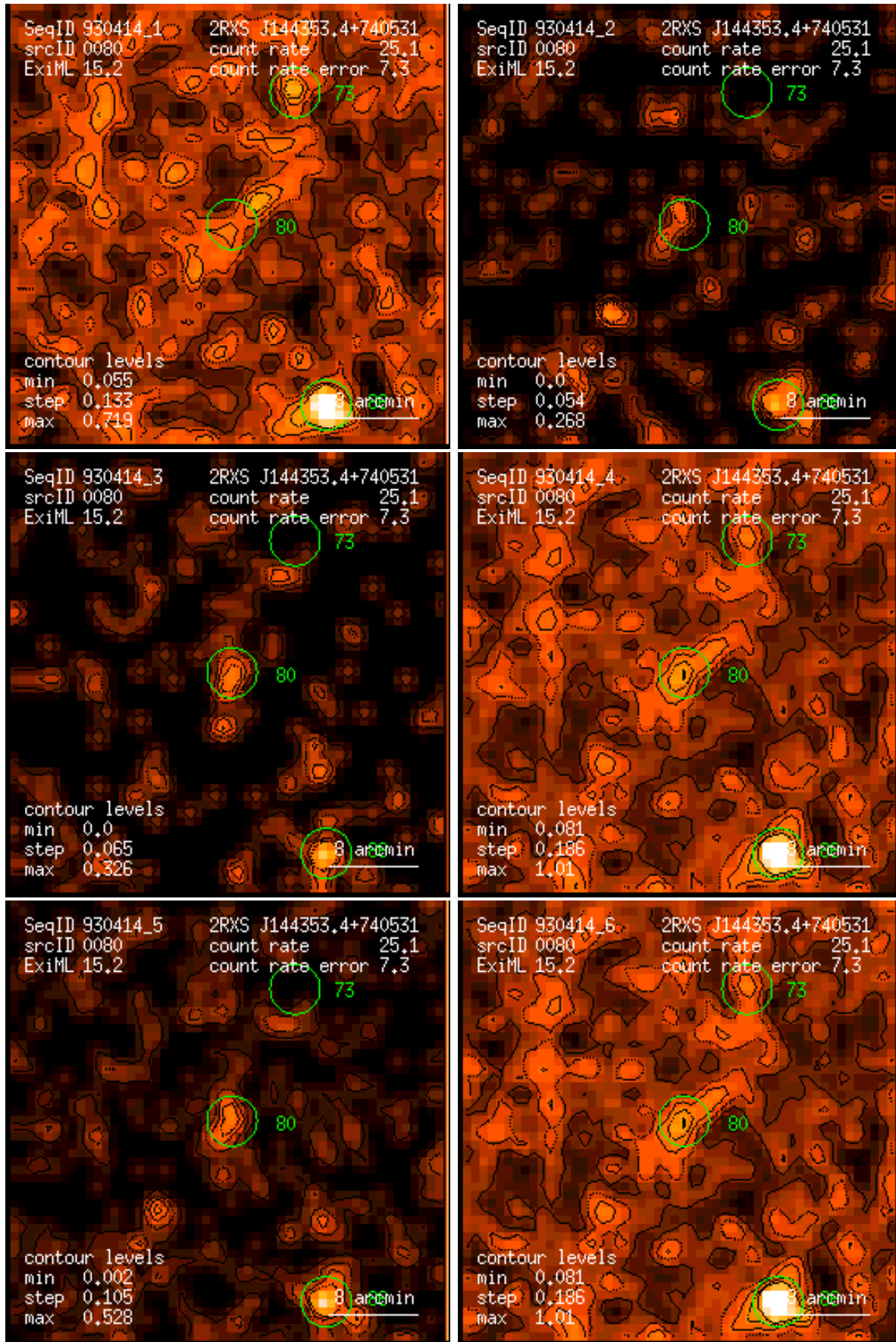
Figure 80: RASS 930414: detection 0080: band rate images, Gaussian filter: (1) PSPC channels 11 – 41, (2) 52 – 90, (3) 91 – 201, (4) 11 – 235, (5) 52 – 201, (6) 11 – 201. Broad band rates in counts/ks. Band rate contour levels in counts/ks/arcmin 2 .
