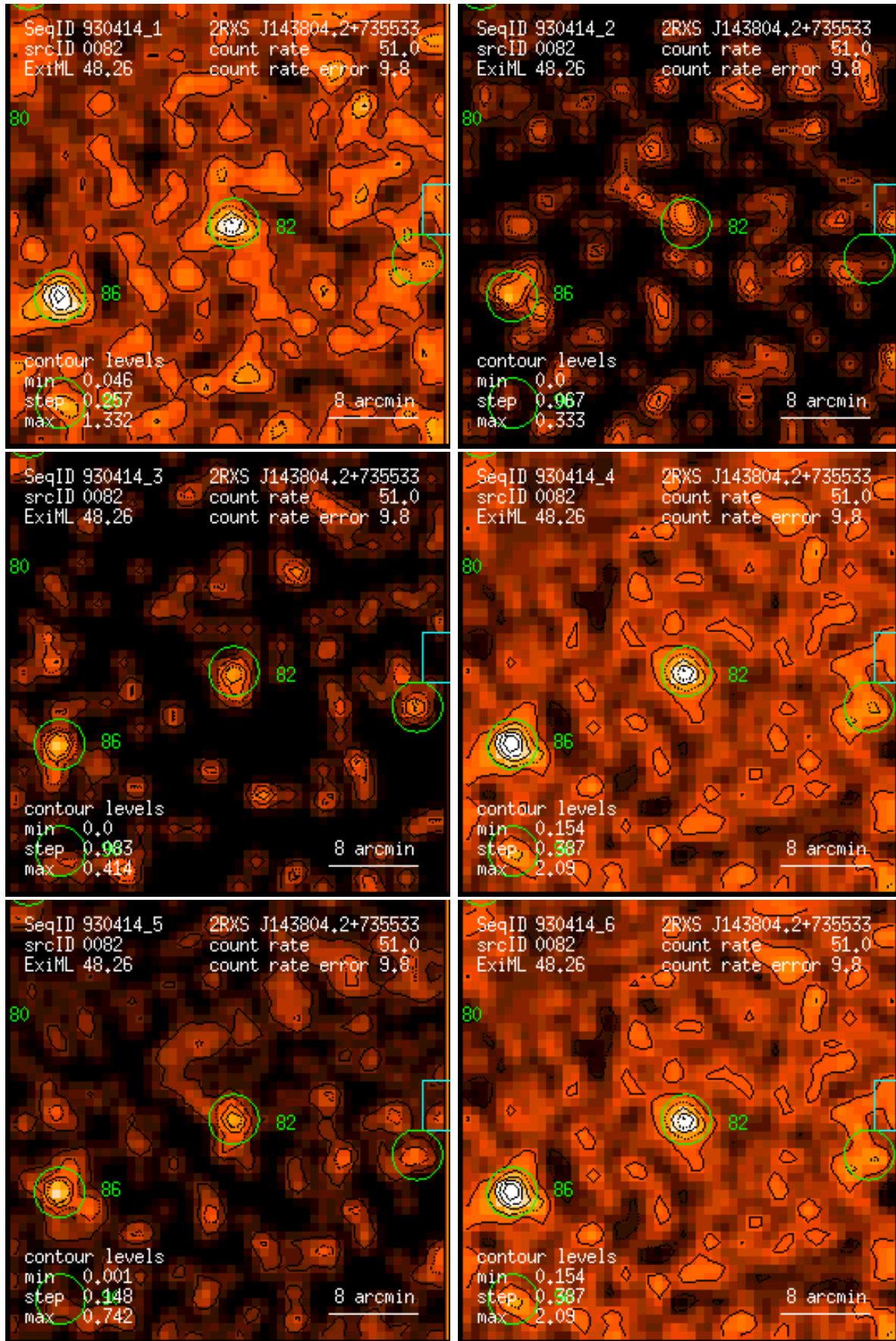
Figure 82: RASS 930414: detection 0082: band rate images, Gaussian filter: (1) PSPC channels 11 – 41, (2) 52 – 90, (3) 91 – 201, (4) 11 – 235, (5) 52 – 201, (6) 11 – 201. Broad band rates in counts/ks. Band rate contour levels in counts/ks/arcmin 2 .
