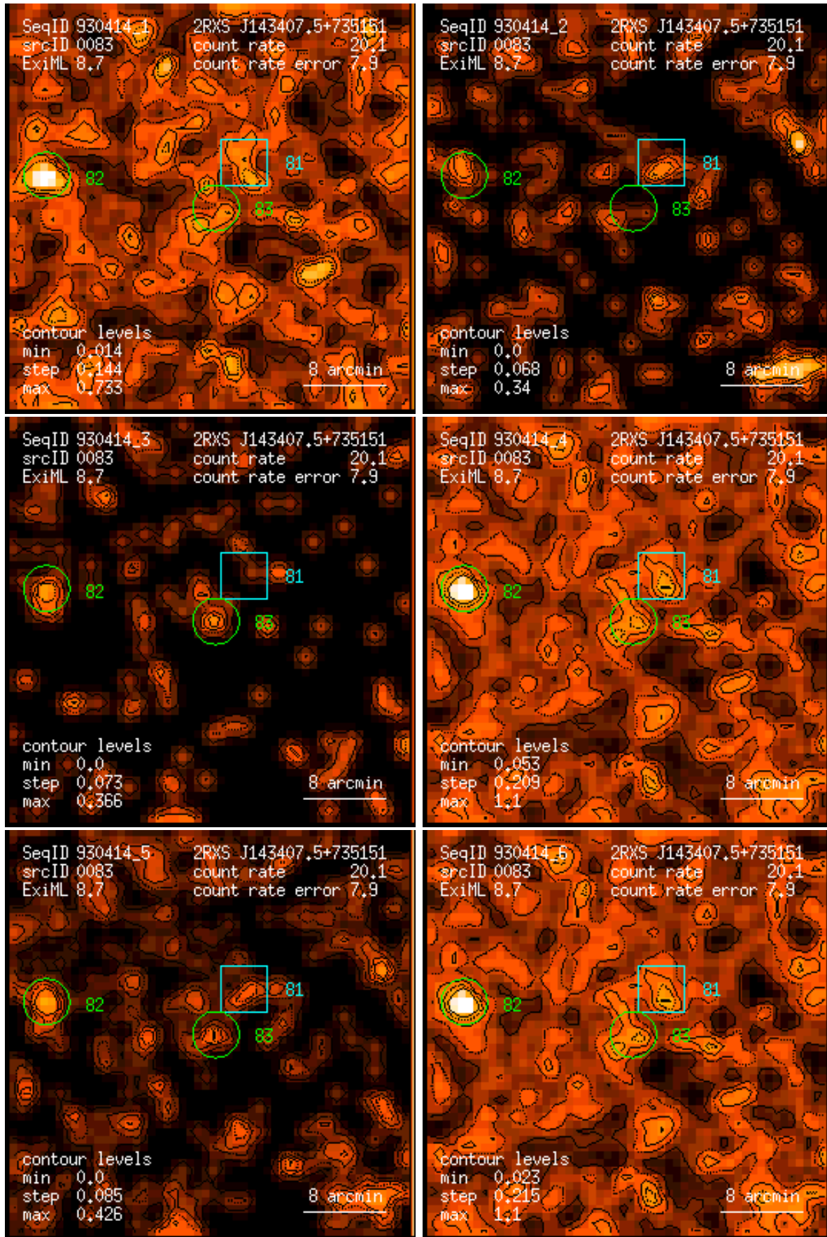
Figure 83: RASS 930414: detection 0083: band rate images, Gaussian filter: (1) PSPC channels 11 – 41, (2) 52 – 90, (3) 91 – 201, (4) 11 – 235, (5) 52 – 201, (6) 11 – 201. Broad band rates in counts/ks. Band rate contour levels in counts/ks/arcmin 2 .
