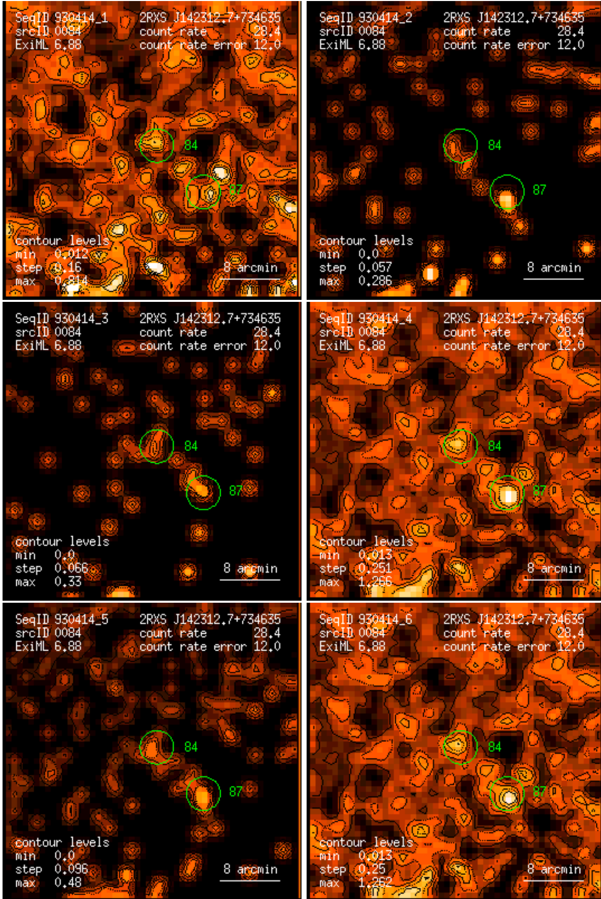
Figure 84: RASS 930414: detection 0084: band rate images, Gaussian filter: (1) PSPC channels 11 – 41, (2) 52 – 90, (3) 91 – 201, (4) 11 – 235, (5) 52 – 201, (6) 11 – 201. Broad band rates in counts/ks. Band rate contour levels in counts/ks/arcmin 2 .
