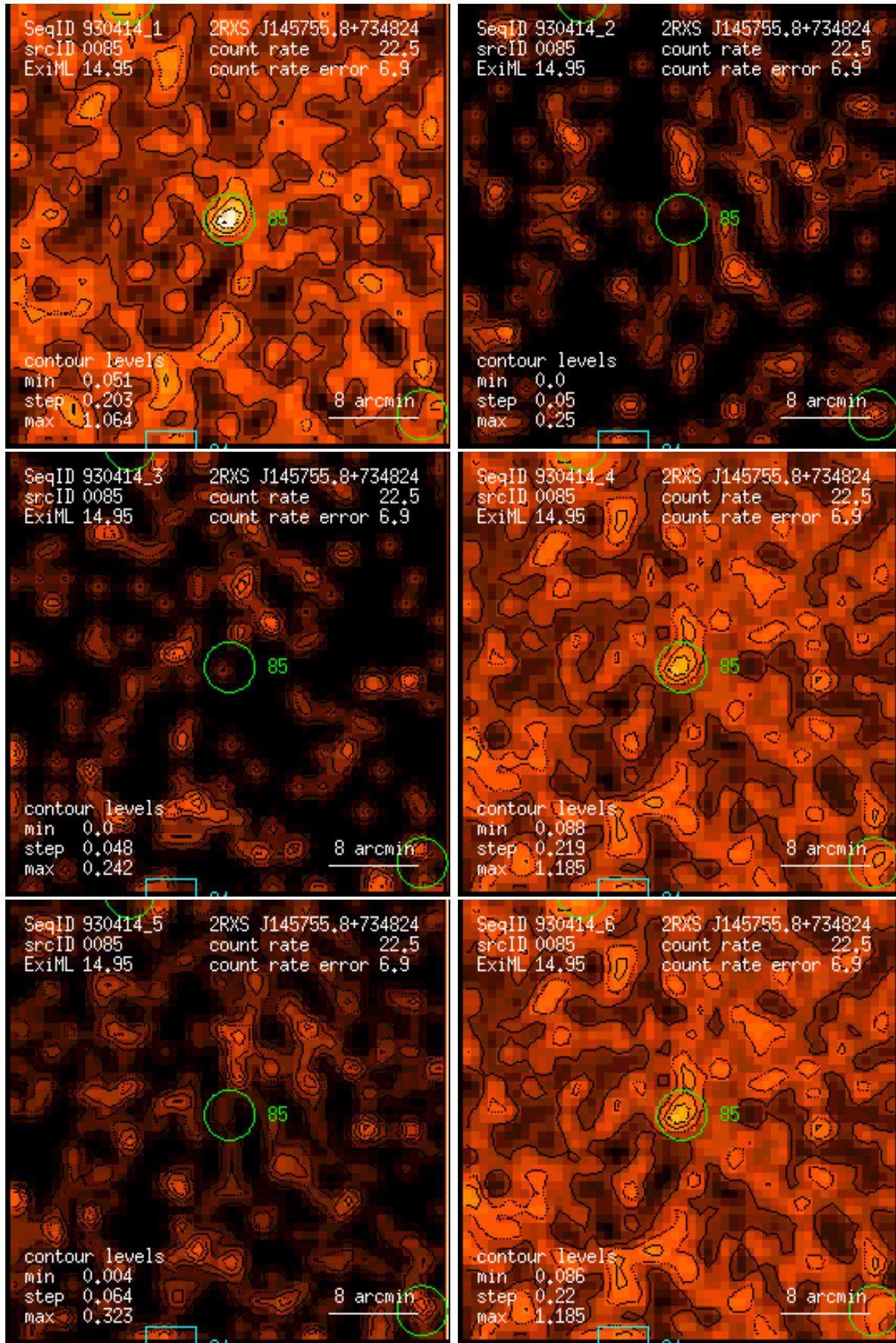
Figure 85: RASS 930414: detection 0085: band rate images, Gaussian filter: (1) PSPC channels 11 – 41, (2) 52 – 90, (3) 91 – 201, (4) 11 – 235, (5) 52 – 201, (6) 11 – 201. Broad band rates in counts/ks. Band rate contour levels in counts/ks/arcmin 2 .
