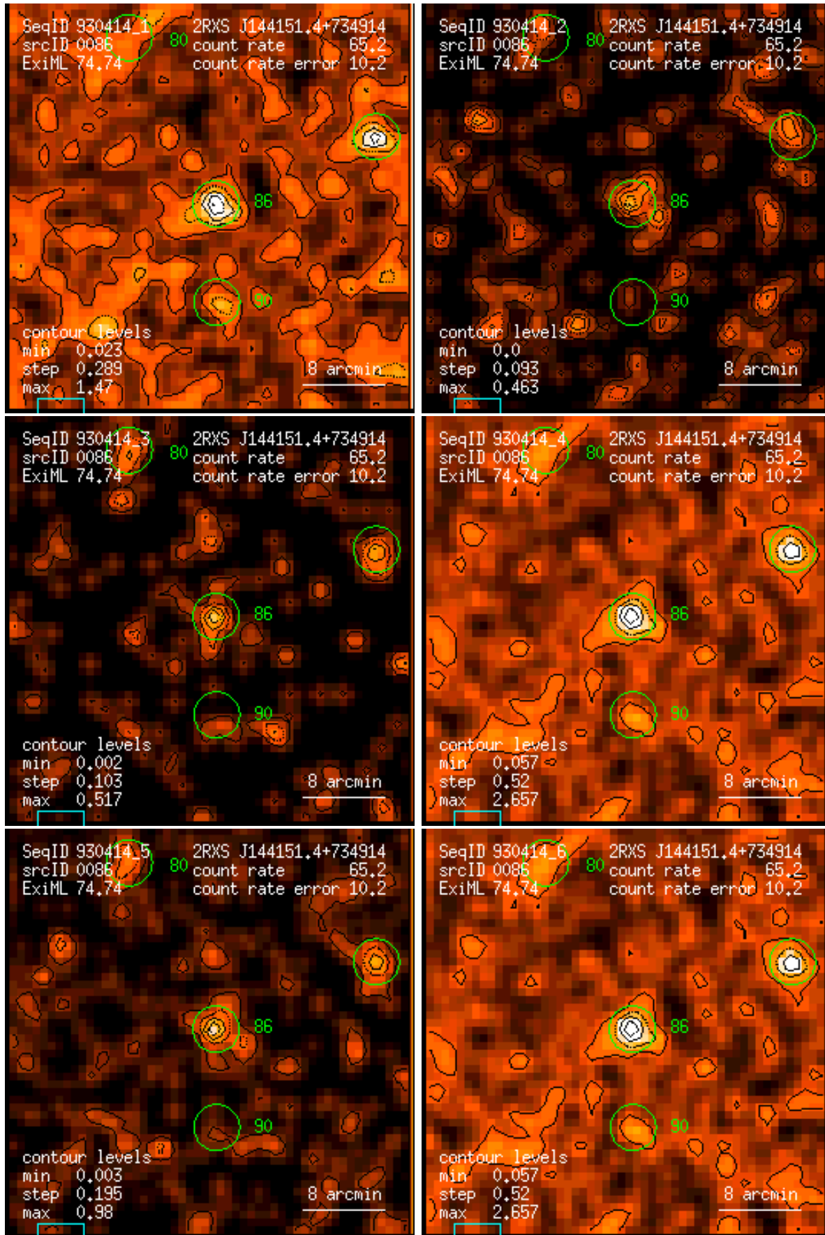
Figure 86: RASS 930414: detection 0086: band rate images, Gaussian filter: (1) PSPC channels 11 – 41, (2) 52 – 90, (3) 91 – 201, (4) 11 – 235, (5) 52 – 201, (6) 11 – 201. Broad band rates in counts/ks. Band rate contour levels in counts/ks/arcmin 2 .
