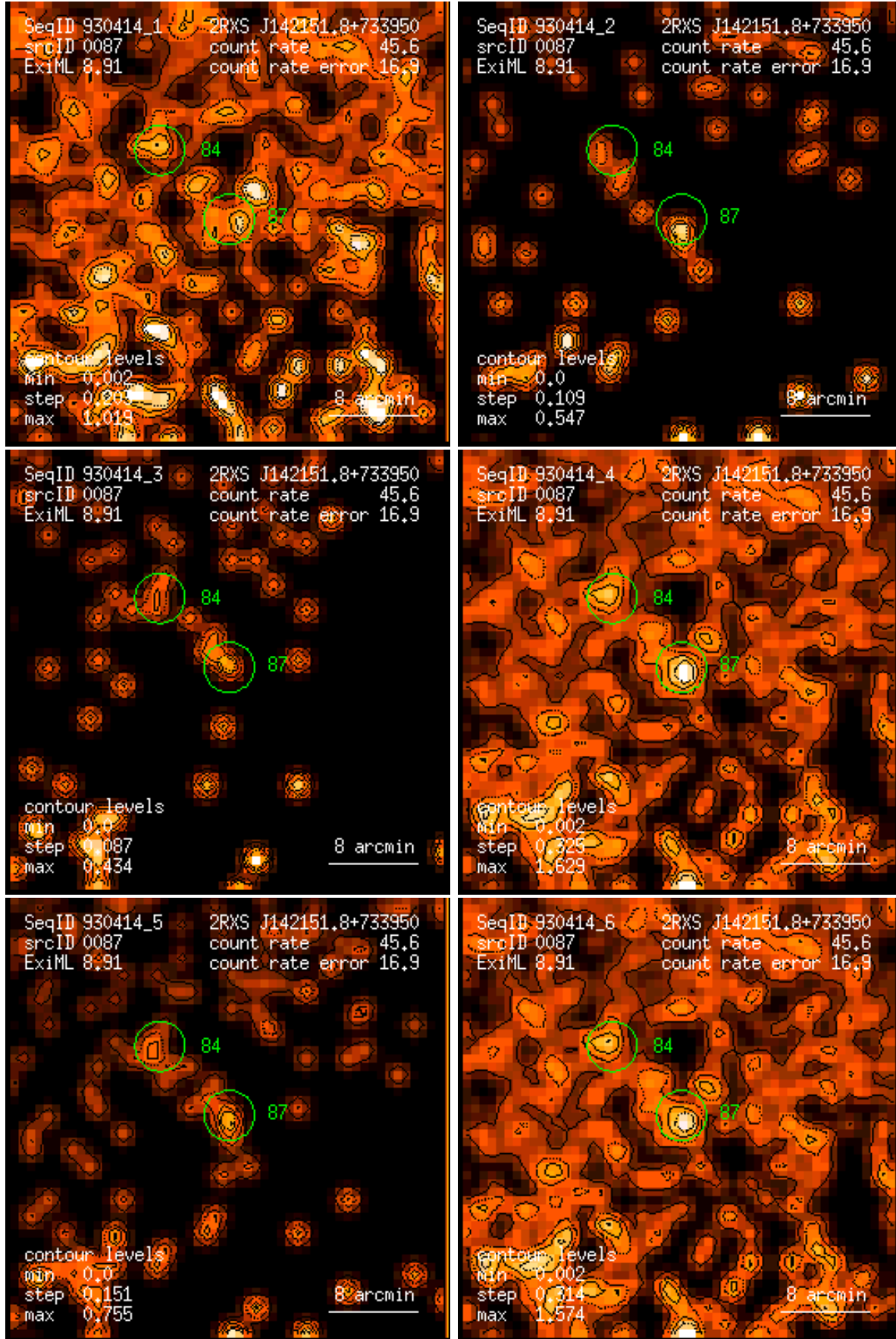
Figure 87: RASS 930414: detection 0087: band rate images, Gaussian filter: (1) PSPC channels 11 – 41, (2) 52 – 90, (3) 91 – 201, (4) 11 – 235, (5) 52 – 201, (6) 11 – 201. Broad band rates in counts/ks. Band rate contour levels in counts/ks/arcmin 2 .
