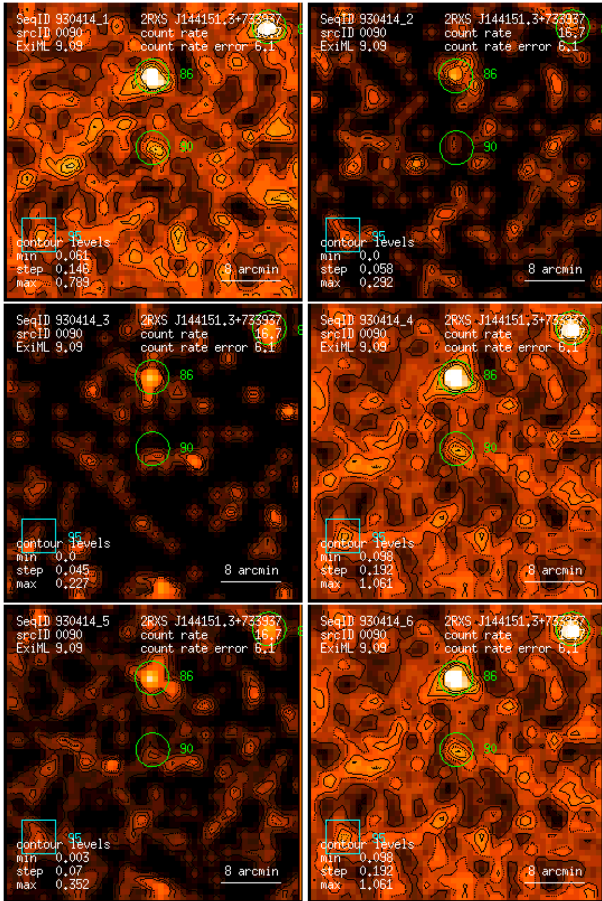
Figure 90: RASS 930414: detection 0090: band rate images, Gaussian filter: (1) PSPC channels 11 – 41, (2) 52 – 90, (3) 91 – 201, (4) 11 – 235, (5) 52 – 201, (6) 11 – 201. Broad band rates in counts/ks. Band rate contour levels in counts/ks/arcmin 2 .
