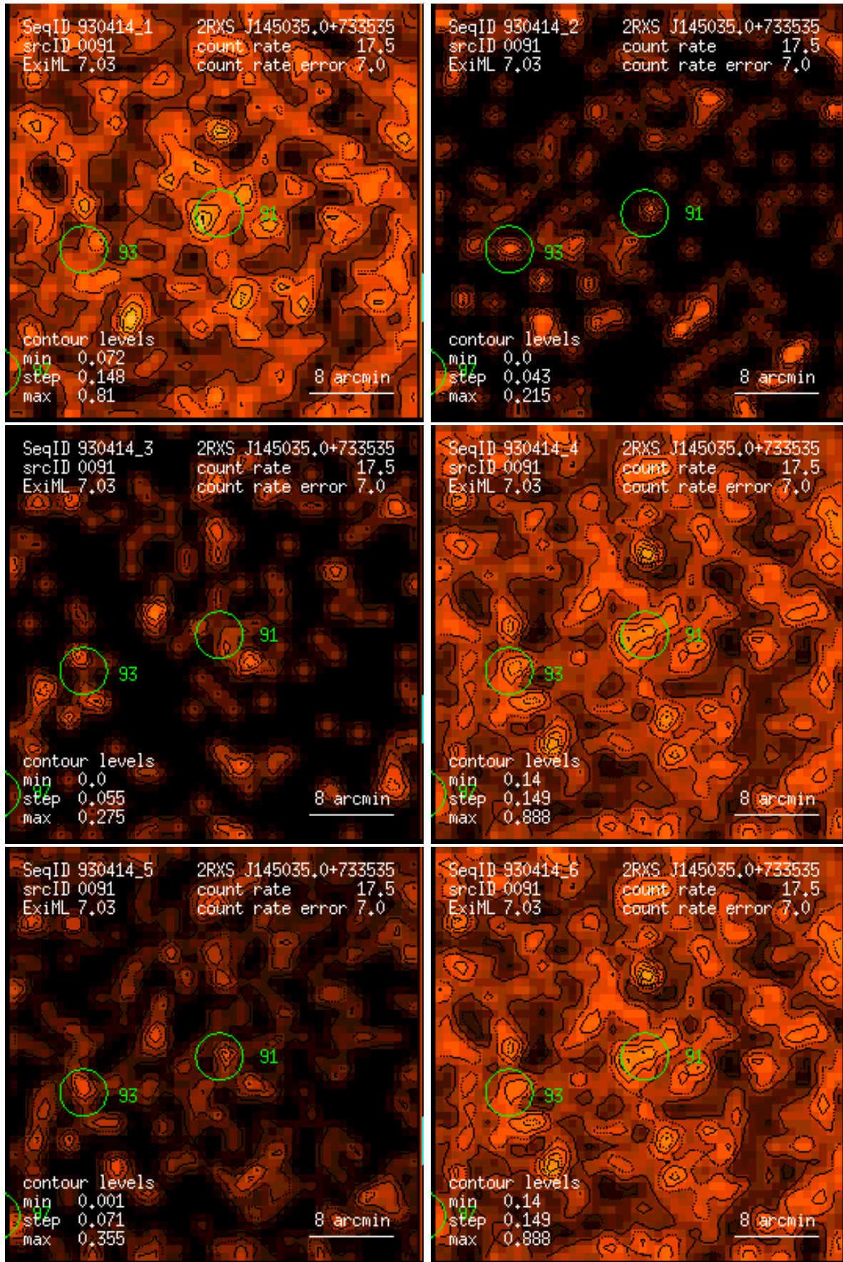
Figure 91: RASS 930414: detection 0091: band rate images, Gaussian filter: (1) PSPC channels 11 – 41, (2) 52 – 90, (3) 91 – 201, (4) 11 – 235, (5) 52 – 201, (6) 11 – 201. Broad band rates in counts/ks. Band rate contour levels in counts/ks/arcmin 2 .
