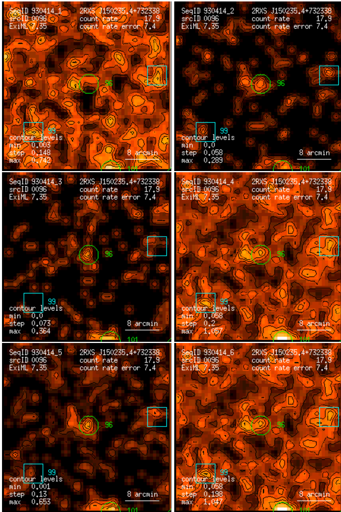
Figure 96: RASS 930414: detection 0096: band rate images, Gaussian filter: (1) PSPC channels 11 – 41, (2) 52 – 90, (3) 91 – 201, (4) 11 – 235, (5) 52 – 201, (6) 11 – 201. Broad band rates in counts/ks. Band rate contour levels in counts/ks/arcmin 2 .
