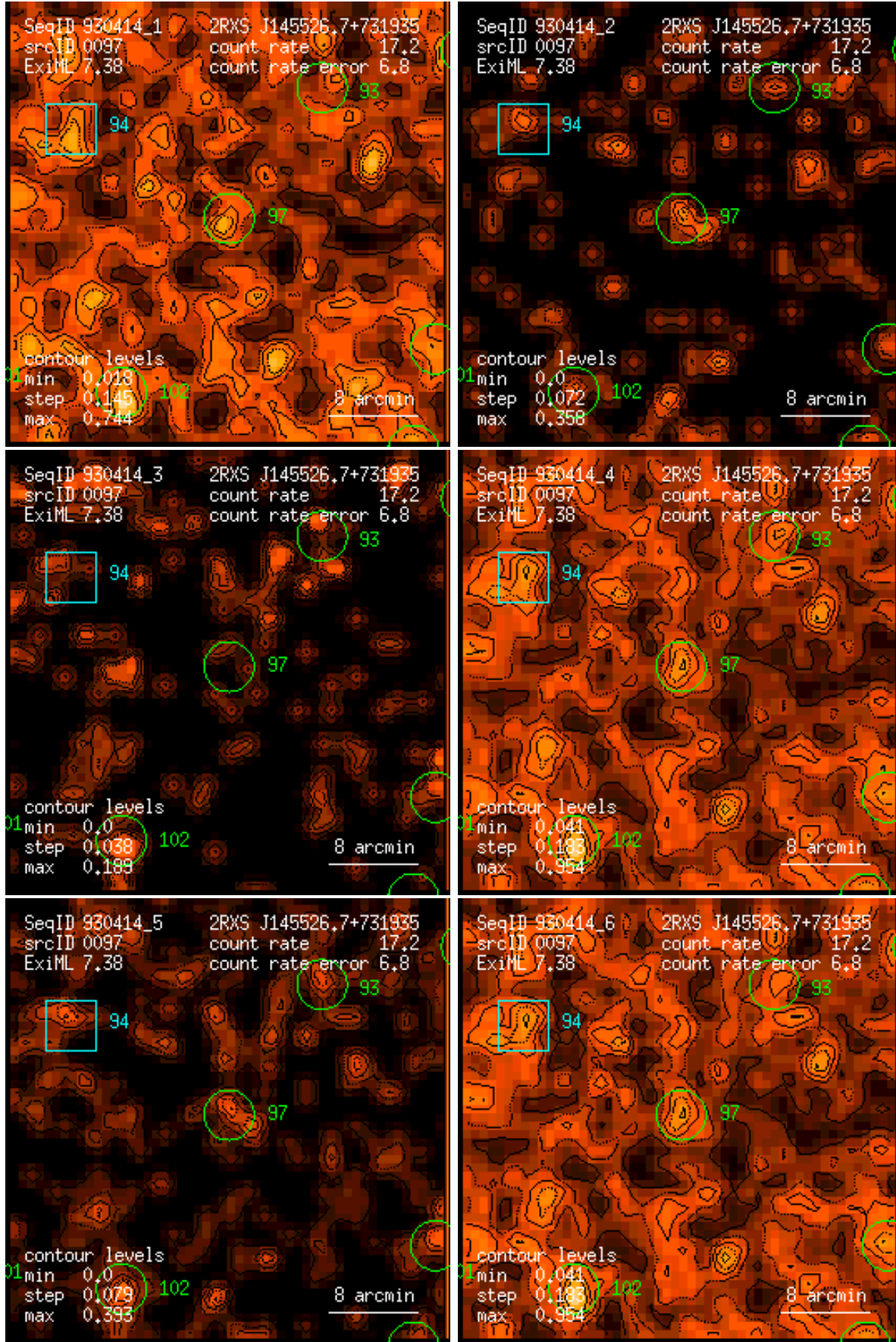
Figure 97: RASS 930414: detection 0097: band rate images, Gaussian filter: (1) PSPC channels 11 – 41, (2) 52 – 90, (3) 91 – 201, (4) 11 – 235, (5) 52 – 201, (6) 11 – 201. Broad band rates in counts/ks. Band rate contour levels in counts/ks/arcmin 2 .
