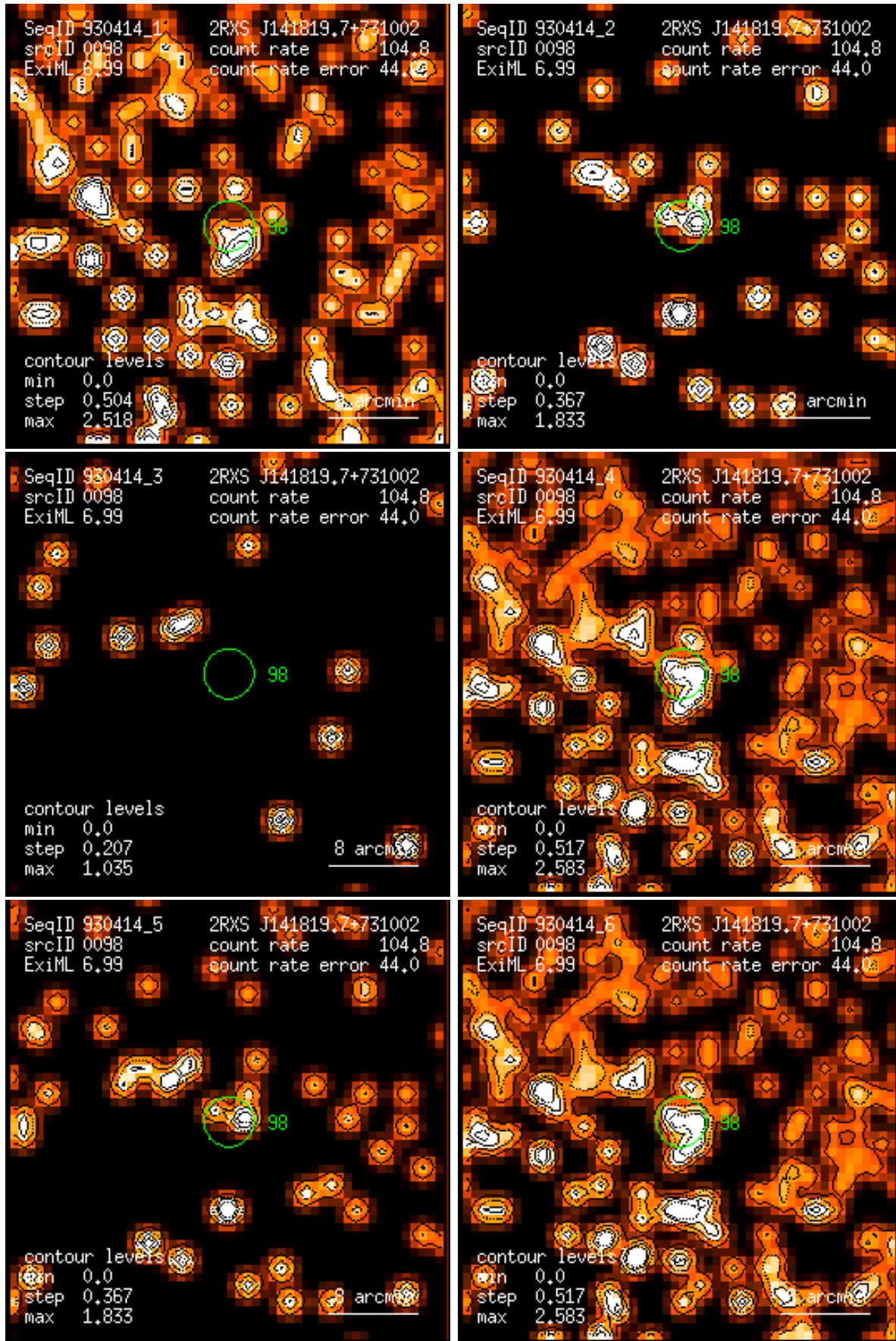
Figure 98: RASS 930414: detection 0098: band rate images, Gaussian filter: (1) PSPC channels 11 – 41, (2) 52 – 90, (3) 91 – 201, (4) 11 – 235, (5) 52 – 201, (6) 11 – 201. Broad band rates in counts/ks. Band rate contour levels in counts/ks/arcmin 2 .
