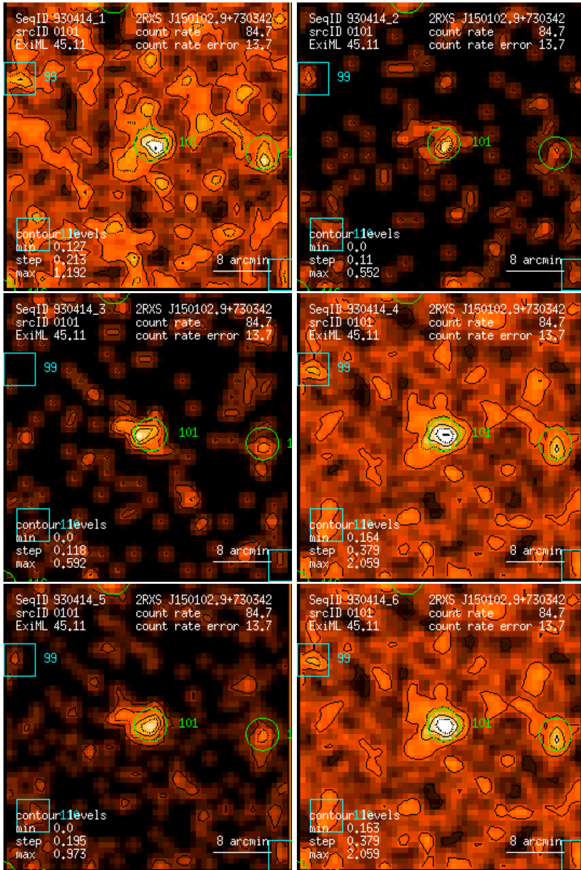
Figure 101: RASS 930414: detection 0101: band rate images, Gaussian filter: (1) PSPC channels 11 – 41, (2) 52 – 90, (3) 91 – 201, (4) 11 – 235, (5) 52 – 201, (6) 11 – 201. Broad band rates in counts/ks. Band rate contour levels in counts/ks/arcmin 2 .
