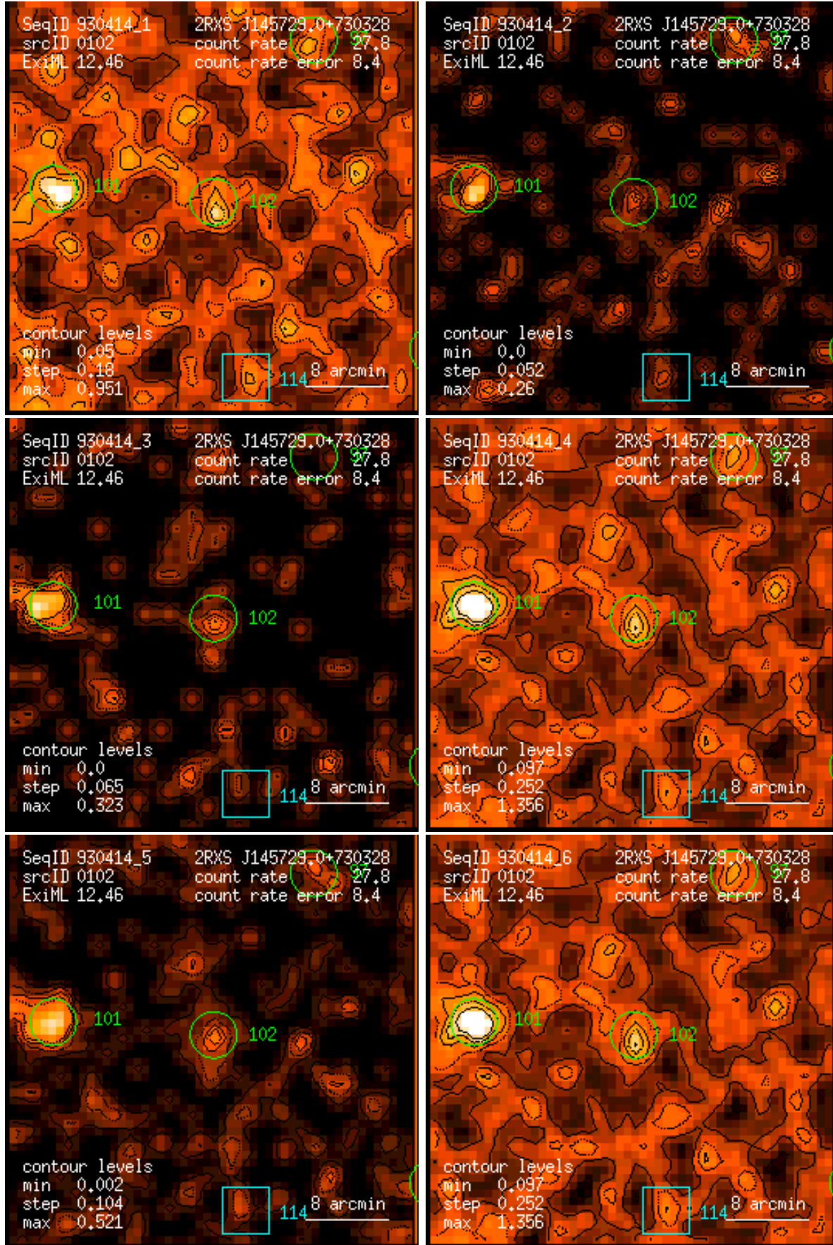
Figure 102: RASS 930414: detection 0102: band rate images, Gaussian filter: (1) PSPC channels 11 – 41, (2) 52 – 90, (3) 91 – 201, (4) 11 – 235, (5) 52 – 201, (6) 11 – 201. Broad band rates in counts/ks. Band rate contour levels in counts/ks/arcmin 2 .
