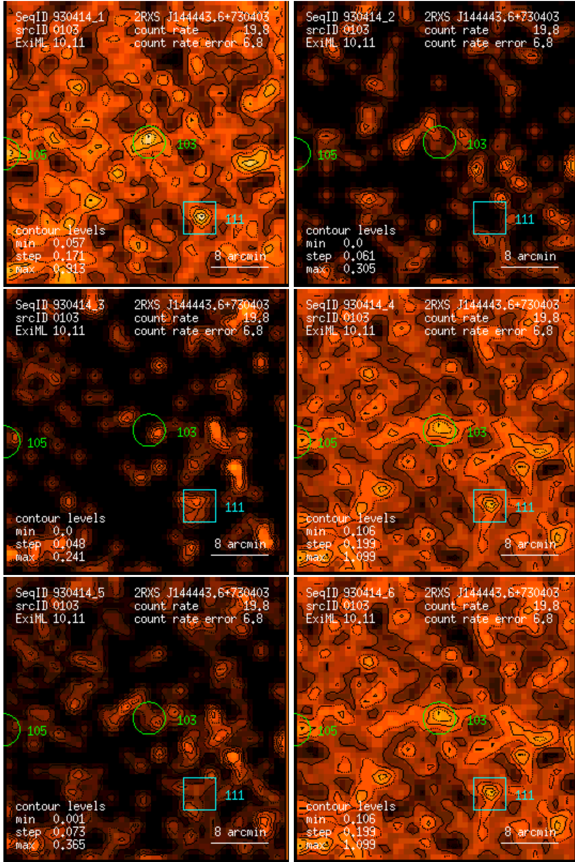
Figure 103: RASS 930414: detection 0103: band rate images, Gaussian filter: (1) PSPC channels 11 – 41, (2) 52 – 90, (3) 91 – 201, (4) 11 – 235, (5) 52 – 201, (6) 11 – 201. Broad band rates in counts/ks. Band rate contour levels in counts/ks/arcmin 2 .
