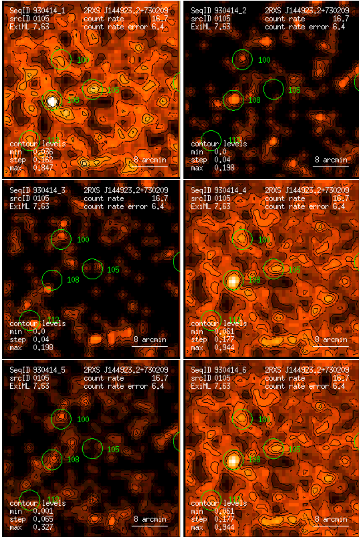
Figure 105: RASS 930414: detection 0105: band rate images, Gaussian filter: (1) PSPC channels 11 – 41, (2) 52 – 90, (3) 91 – 201, (4) 11 – 235, (5) 52 – 201, (6) 11 – 201. Broad band rates in counts/ks. Band rate contour levels in counts/ks/arcmin 2 .
