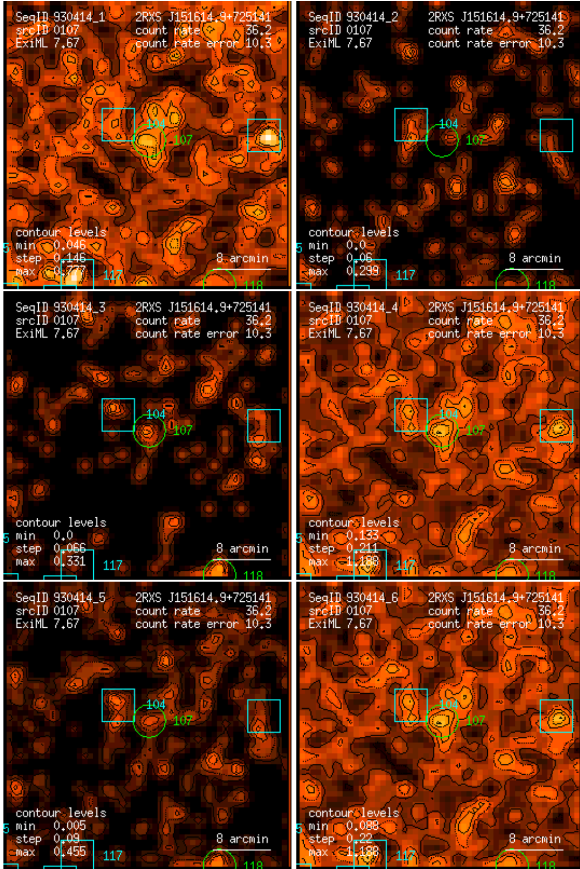
Figure 107: RASS 930414: detection 0107: band rate images, Gaussian filter: (1) PSPC channels 11 – 41, (2) 52 – 90, (3) 91 – 201, (4) 11 – 235, (5) 52 – 201, (6) 11 – 201. Broad band rates in counts/ks. Band rate contour levels in counts/ks/arcmin 2 .
