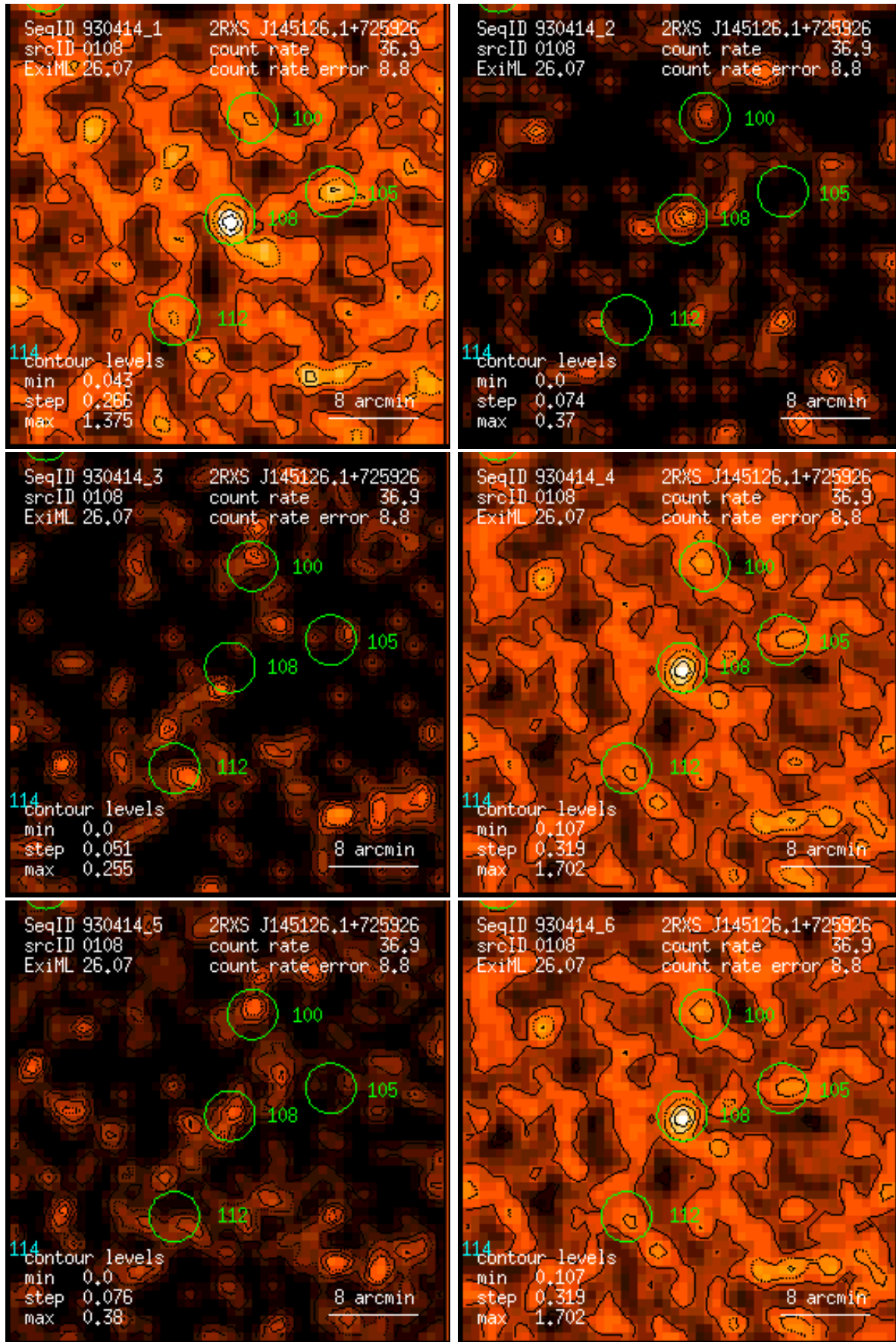
Figure 108: RASS 930414: detection 0108: band rate images, Gaussian filter: (1) PSPC channels 11 – 41, (2) 52 – 90, (3) 91 – 201, (4) 11 – 235, (5) 52 – 201, (6) 11 – 201. Broad band rates in counts/ks. Band rate contour levels in counts/ks/arcmin 2 .
