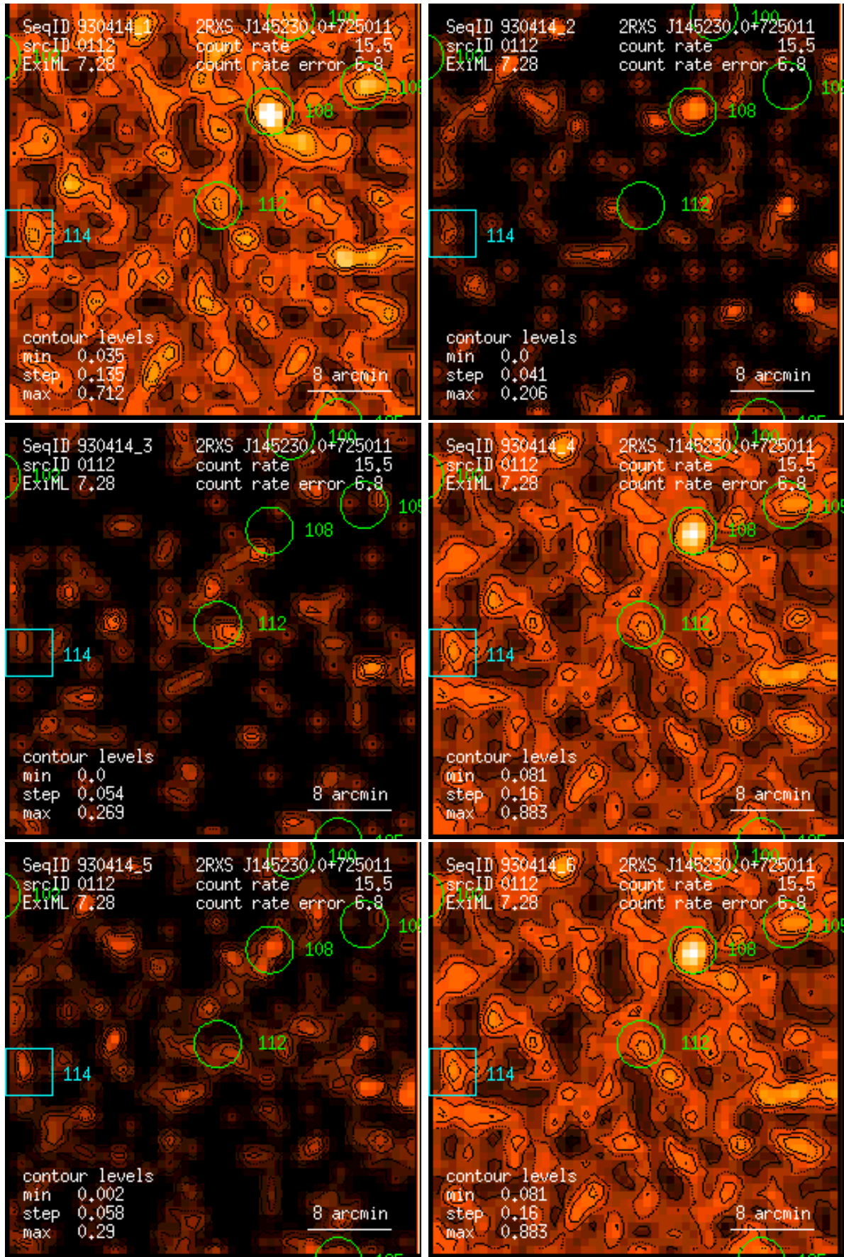
Figure 112: RASS 930414: detection 0112: band rate images, Gaussian filter: (1) PSPC channels 11 – 41, (2) 52 – 90, (3) 91 – 201, (4) 11 – 235, (5) 52 – 201, (6) 11 – 201. Broad band rates in counts/ks. Band rate contour levels in counts/ks/arcmin 2 .
