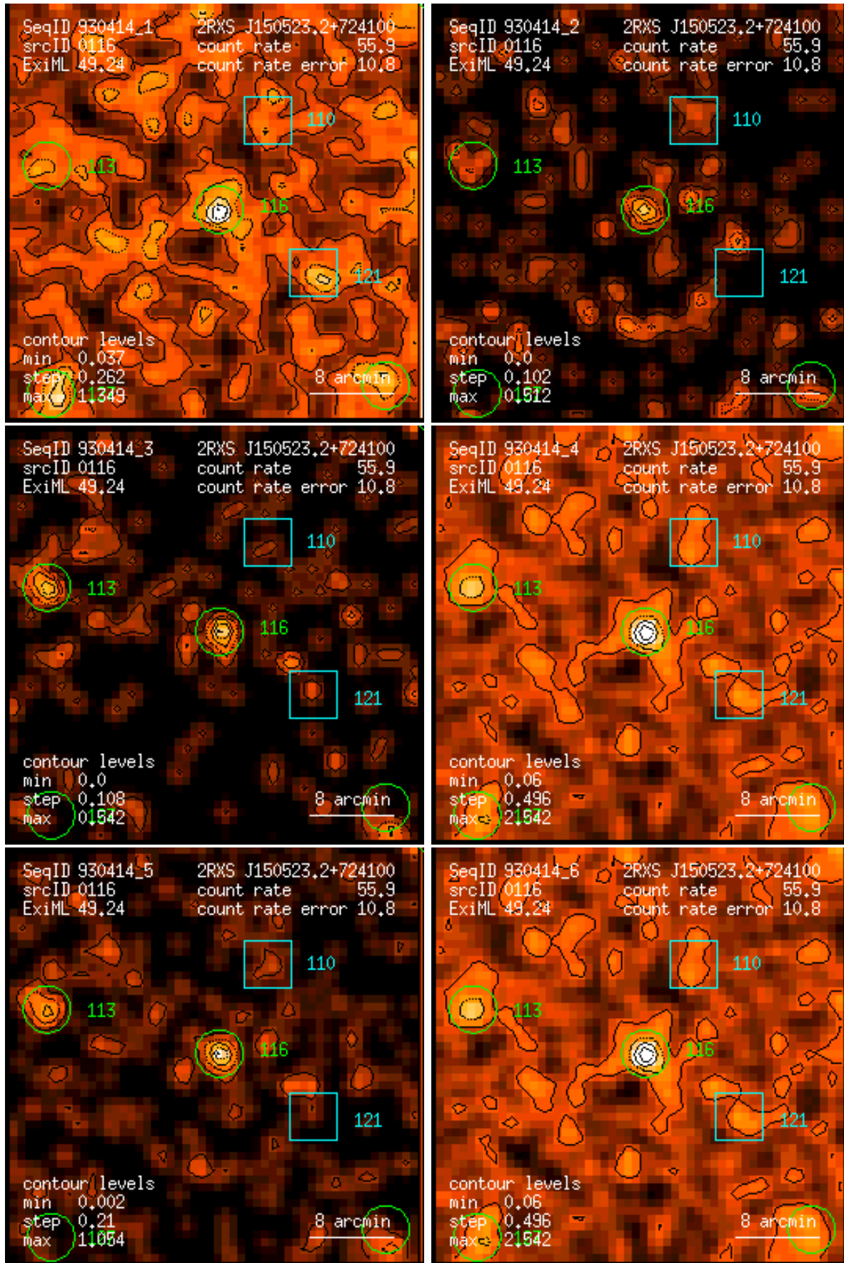
Figure 116: RASS 930414: detection 0116: band rate images, Gaussian filter: (1) PSPC channels 11 – 41, (2) 52 – 90, (3) 91 – 201, (4) 11 – 235, (5) 52 – 201, (6) 11 – 201. Broad band rates in counts/ks. Band rate contour levels in counts/ks/arcmin 2 .
