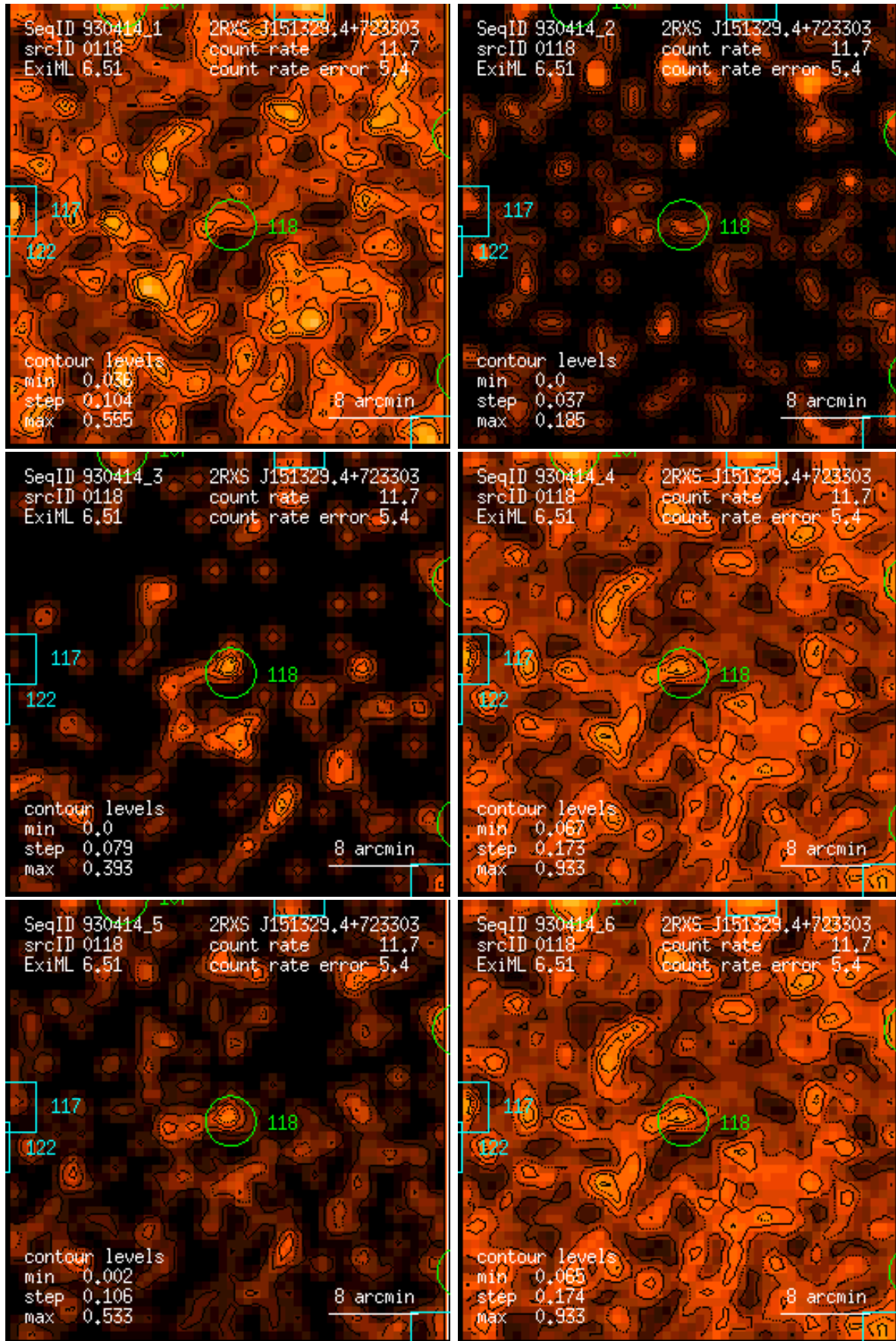
Figure 118: RASS 930414: detection 0118: band rate images, Gaussian filter: (1) PSPC channels 11 – 41, (2) 52 – 90, (3) 91 – 201, (4) 11 – 235, (5) 52 – 201, (6) 11 – 201. Broad band rates in counts/ks. Band rate contour levels in counts/ks/arcmin 2 .
