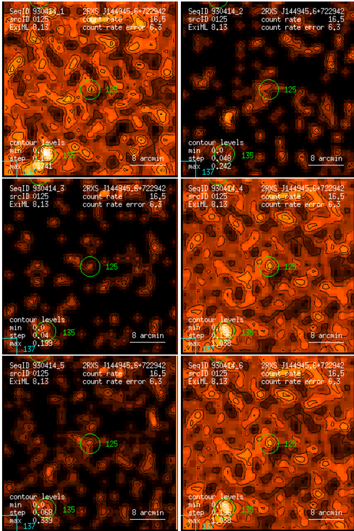
Figure 125: RASS 930414: detection 0125: band rate images, Gaussian filter: (1) PSPC channels 11 – 41, (2) 52 – 90, (3) 91 – 201, (4) 11 – 235, (5) 52 – 201, (6) 11 – 201. Broad band rates in counts/ks. Band rate contour levels in counts/ks/arcmin 2 .
