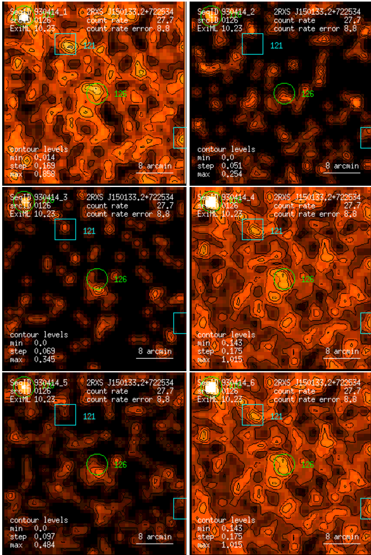
Figure 126: RASS 930414: detection 0126: band rate images, Gaussian filter: (1) PSPC channels 11 – 41, (2) 52 – 90, (3) 91 – 201, (4) 11 – 235, (5) 52 – 201, (6) 11 – 201. Broad band rates in counts/ks. Band rate contour levels in counts/ks/arcmin 2 .
