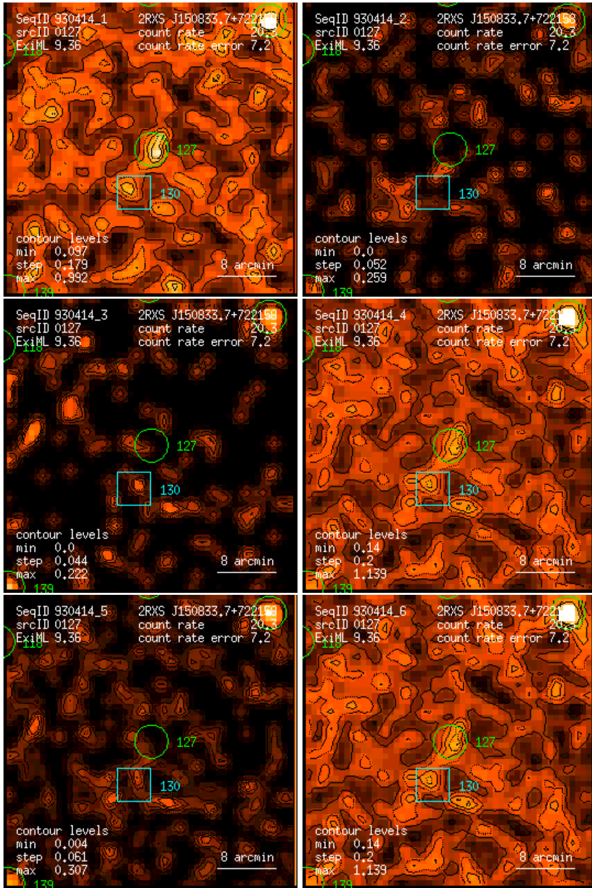
Figure 127: RASS 930414: detection 0127: band rate images, Gaussian filter: (1) PSPC channels 11 – 41, (2) 52 – 90, (3) 91 – 201, (4) 11 – 235, (5) 52 – 201, (6) 11 – 201. Broad band rates in counts/ks. Band rate contour levels in counts/ks/arcmin 2 .
