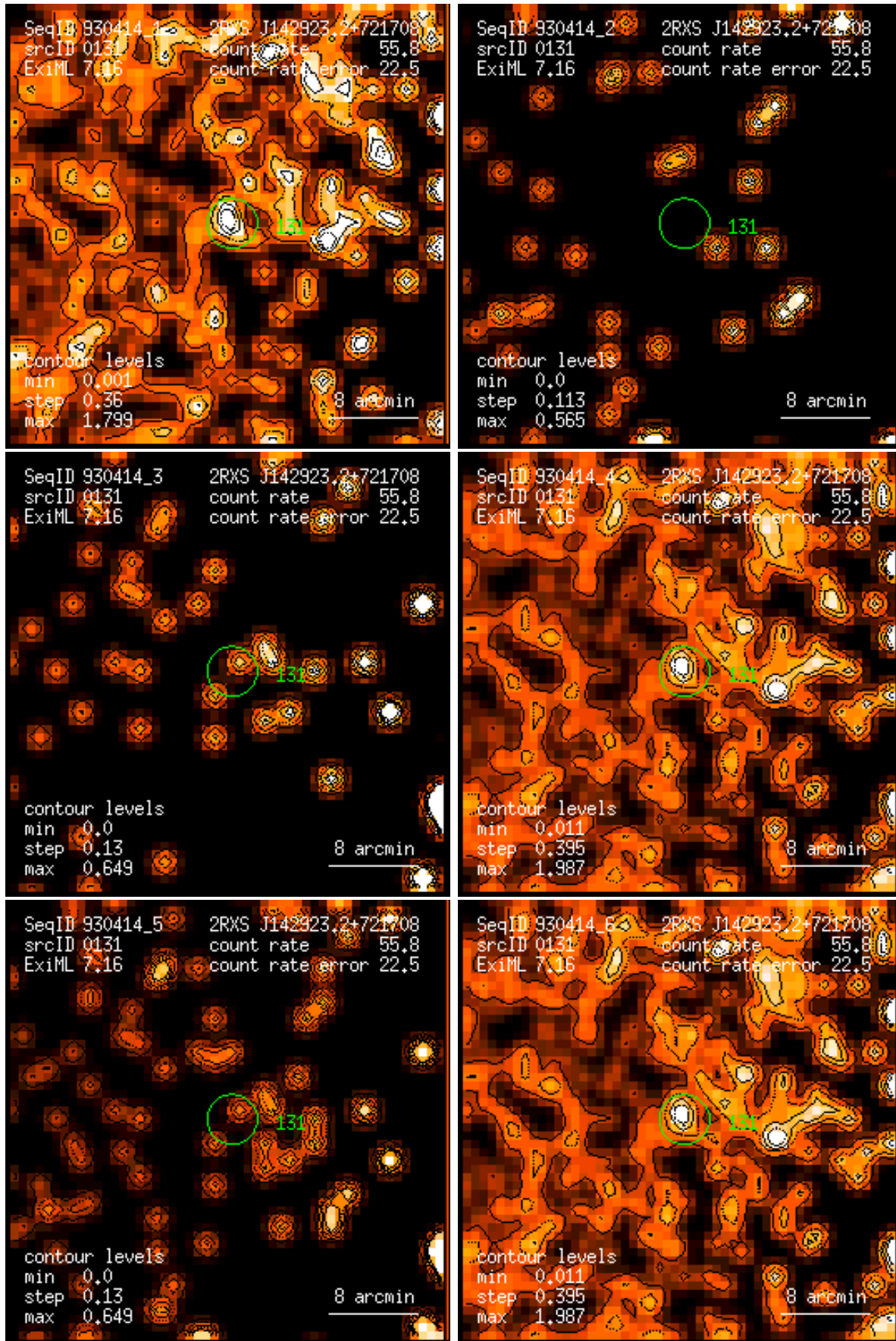
Figure 131: RASS 930414: detection 0131: band rate images, Gaussian filter: (1) PSPC channels 11 – 41, (2) 52 – 90, (3) 91 – 201, (4) 11 – 235, (5) 52 – 201, (6) 11 – 201. Broad band rates in counts/ks. Band rate contour levels in counts/ks/arcmin 2 .
