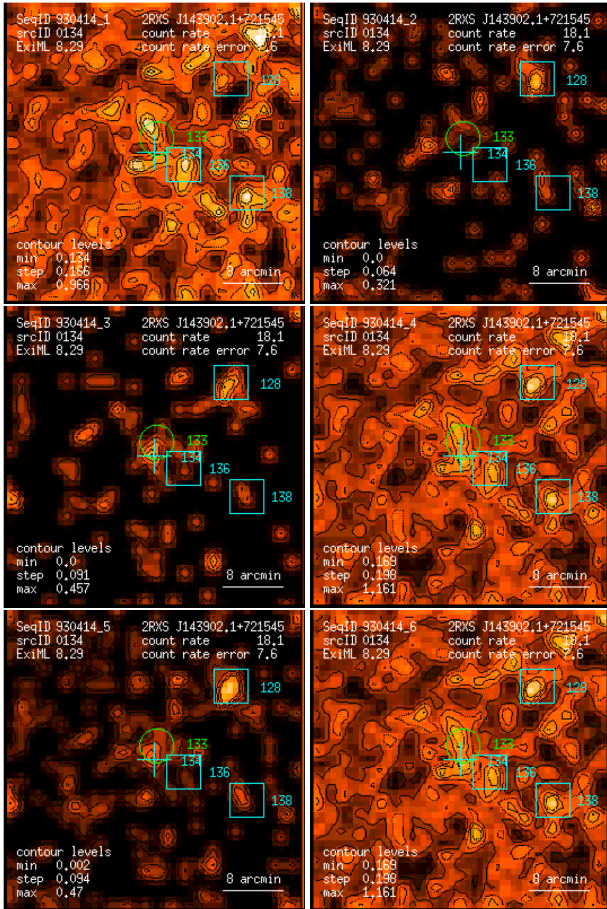
Figure 134: RASS 930414: detection 0134: band rate images, Gaussian filter: (1) PSPC channels 11 – 41, (2) 52 – 90, (3) 91 – 201, (4) 11 – 235, (5) 52 – 201, (6) 11 – 201. Broad band rates in counts/ks. Band rate contour levels in counts/ks/arcmin 2 .
