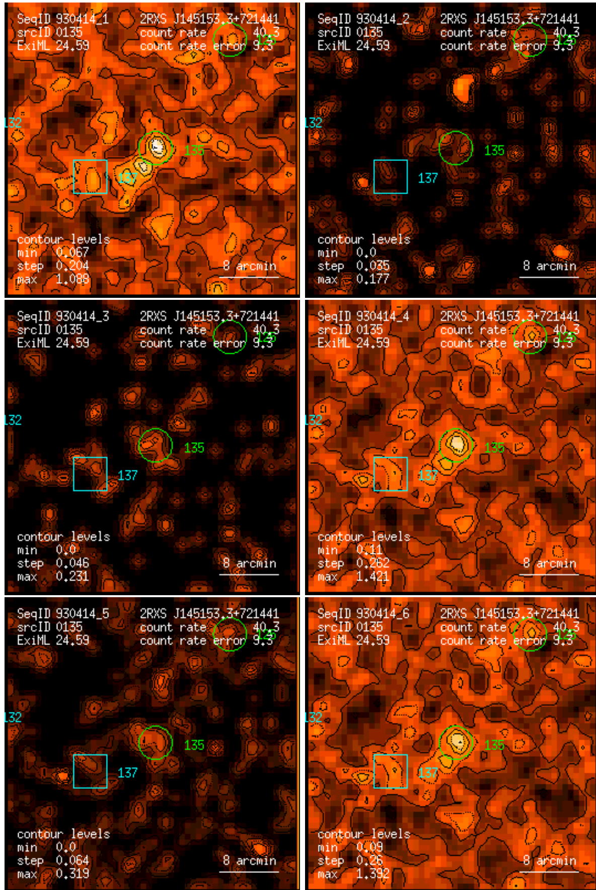
Figure 135: RASS 930414: detection 0135: band rate images, Gaussian filter: (1) PSPC channels 11 – 41, (2) 52 – 90, (3) 91 – 201, (4) 11 – 235, (5) 52 – 201, (6) 11 – 201. Broad band rates in counts/ks. Band rate contour levels in counts/ks/arcmin 2 .
