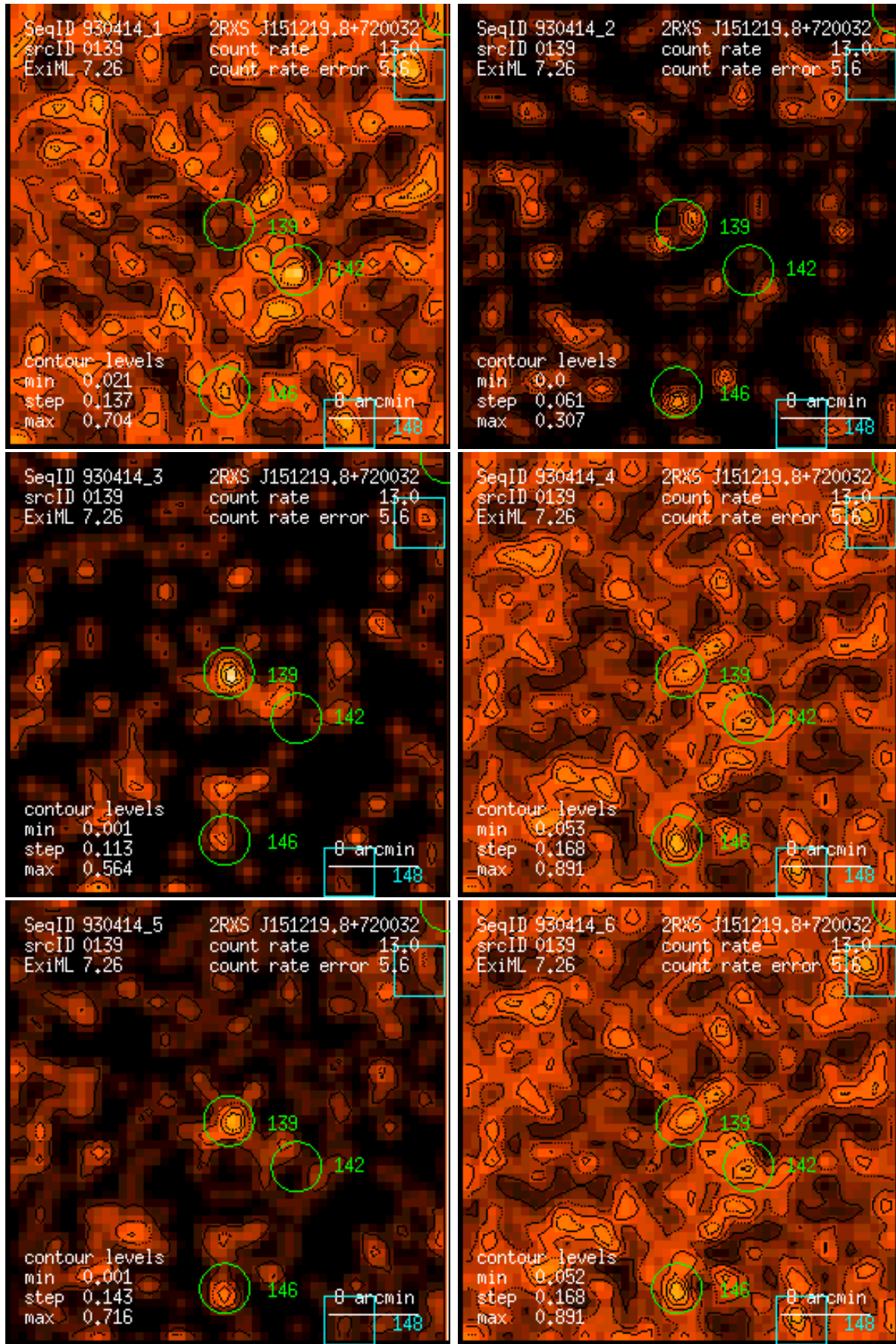
Figure 139: RASS 930414: detection 0139: band rate images, Gaussian filter: (1) PSPC channels 11 – 41, (2) 52 – 90, (3) 91 – 201, (4) 11 – 235, (5) 52 – 201, (6) 11 – 201. Broad band rates in counts/ks. Band rate contour levels in counts/ks/arcmin 2 .
