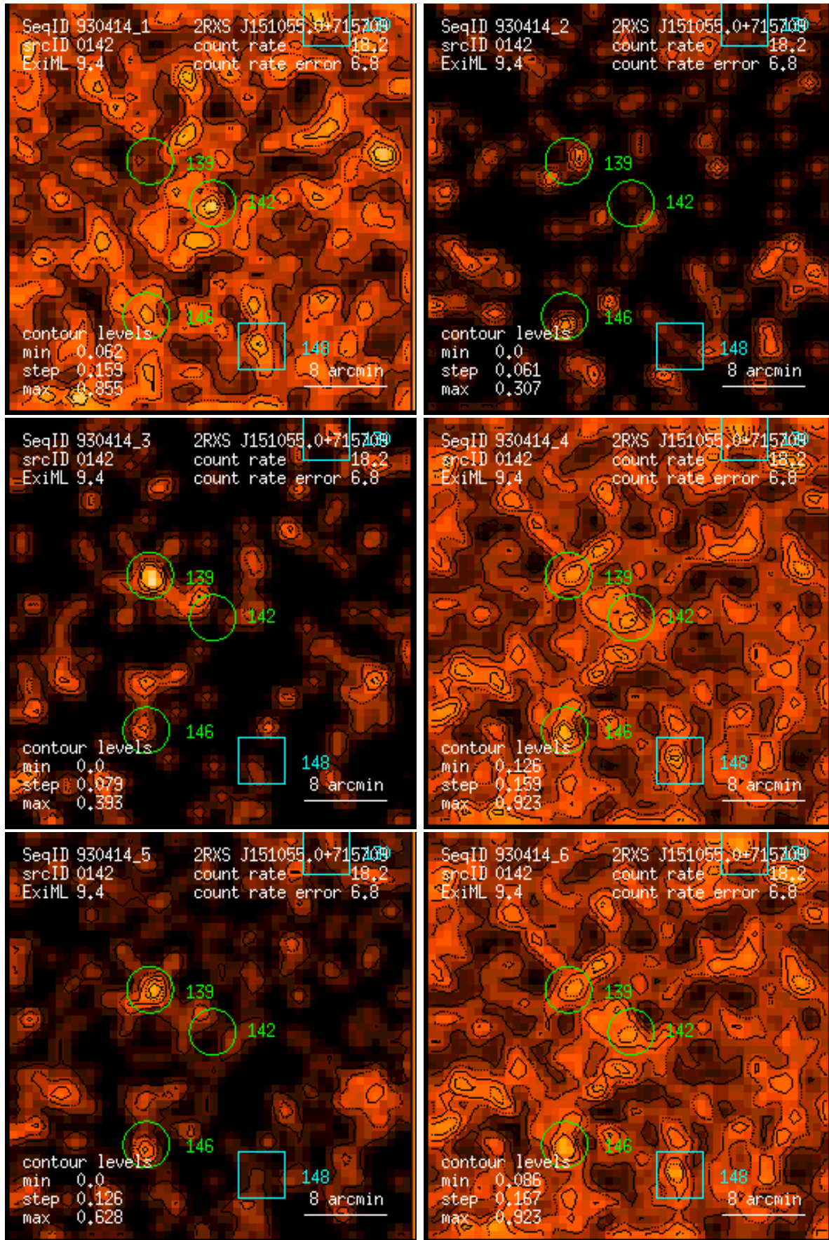
Figure 142: RASS 930414: detection 0142: band rate images, Gaussian filter: (1) PSPC channels 11 – 41, (2) 52 – 90, (3) 91 – 201, (4) 11 – 235, (5) 52 – 201, (6) 11 – 201. Broad band rates in counts/ks. Band rate contour levels in counts/ks/arcmin 2 .
