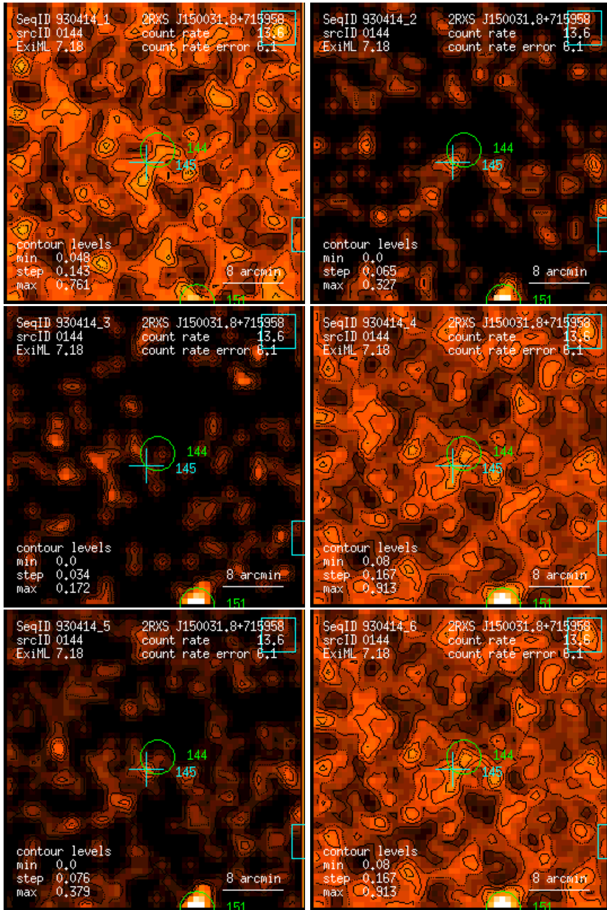
Figure 144: RASS 930414: detection 0144: band rate images, Gaussian filter: (1) PSPC channels 11 – 41, (2) 52 – 90, (3) 91 – 201, (4) 11 – 235, (5) 52 – 201, (6) 11 – 201. Broad band rates in counts/ks. Band rate contour levels in counts/ks/arcmin 2 .
