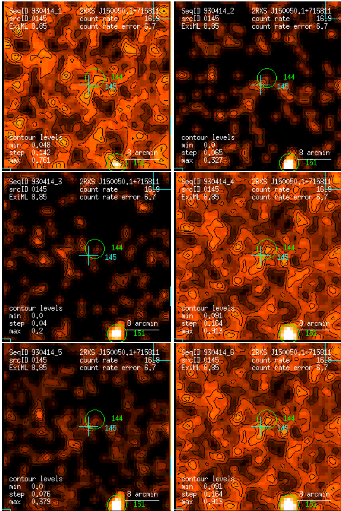
Figure 145: RASS 930414: detection 0145: band rate images, Gaussian filter: (1) PSPC channels 11 – 41, (2) 52 – 90, (3) 91 – 201, (4) 11 – 235, (5) 52 – 201, (6) 11 – 201. Broad band rates in counts/ks. Band rate contour levels in counts/ks/arcmin 2 .
