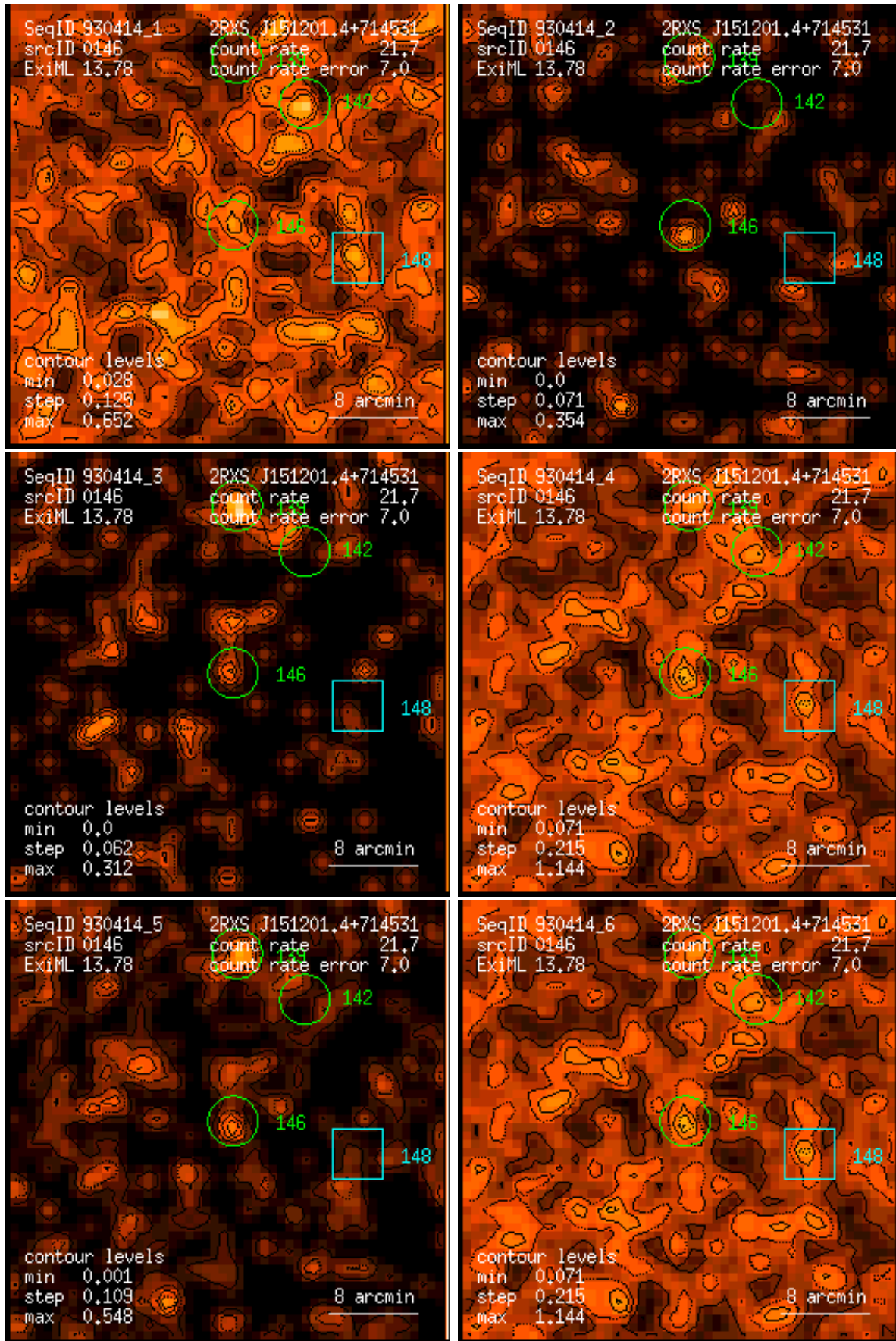
Figure 146: RASS 930414: detection 0146: band rate images, Gaussian filter: (1) PSPC channels 11 – 41, (2) 52 – 90, (3) 91 – 201, (4) 11 – 235, (5) 52 – 201, (6) 11 – 201. Broad band rates in counts/ks. Band rate contour levels in counts/ks/arcmin 2 .
