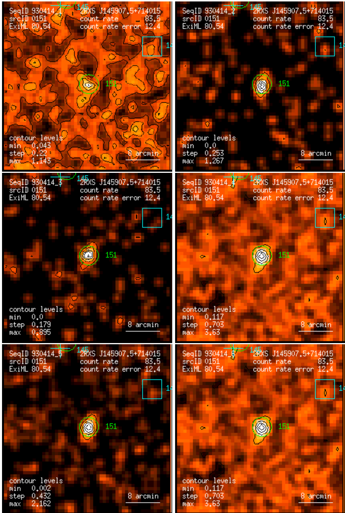
Figure 151: RASS 930414: detection 0151: band rate images, Gaussian filter: (1) PSPC channels 11 – 41, (2) 52 – 90, (3) 91 – 201, (4) 11 – 235, (5) 52 – 201, (6) 11 – 201. Broad band rates in counts/ks. Band rate contour levels in counts/ks/arcmin 2 .
