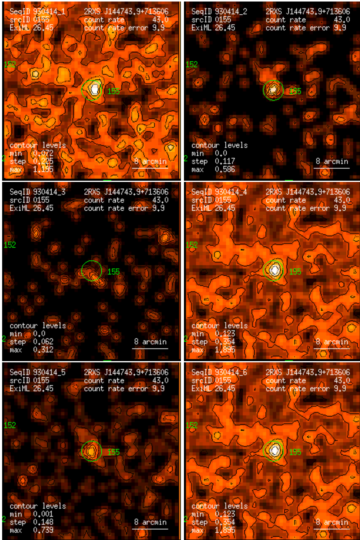
Figure 155: RASS 930414: detection 0155: band rate images, Gaussian filter: (1) PSPC channels 11 – 41, (2) 52 – 90, (3) 91 – 201, (4) 11 – 235, (5) 52 – 201, (6) 11 – 201. Broad band rates in counts/ks. Band rate contour levels in counts/ks/arcmin 2 .
