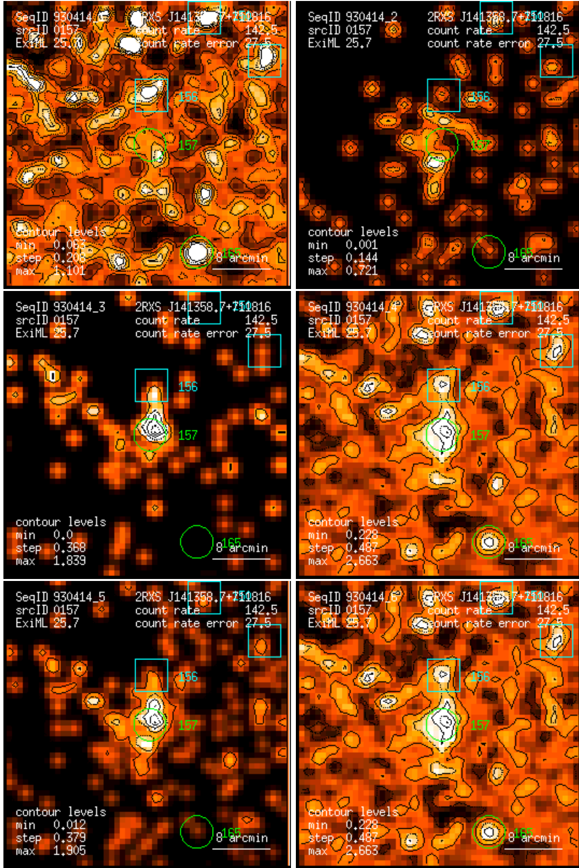
Figure 157: RASS 930414: detection 0157: band rate images, Gaussian filter: (1) PSPC channels 11 – 41, (2) 52 – 90, (3) 91 – 201, (4) 11 – 235, (5) 52 – 201, (6) 11 – 201. Broad band rates in counts/ks. Band rate contour levels in counts/ks/arcmin 2 .
