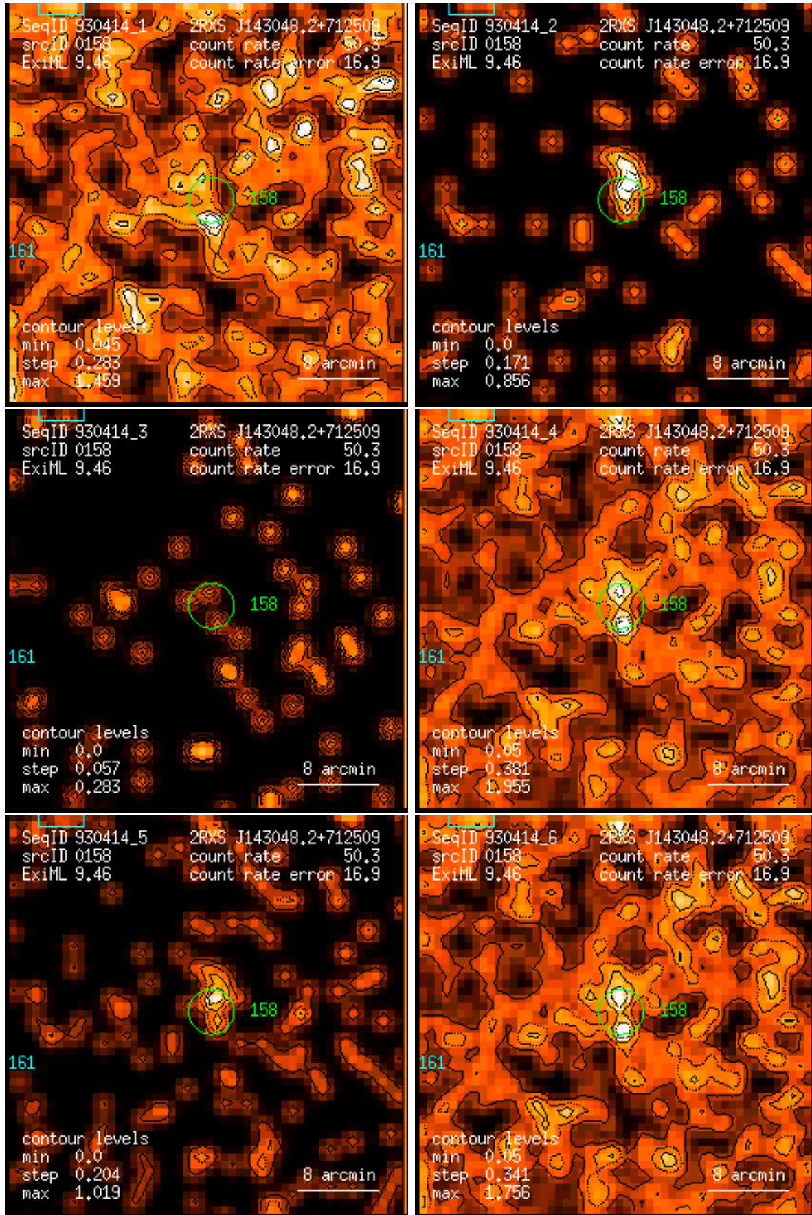
Figure 158: RASS 930414: detection 0158: band rate images, Gaussian filter: (1) PSPC channels 11 – 41, (2) 52 – 90, (3) 91 – 201, (4) 11 – 235, (5) 52 – 201, (6) 11 – 201. Broad band rates in counts/ks. Band rate contour levels in counts/ks/arcmin 2 .
