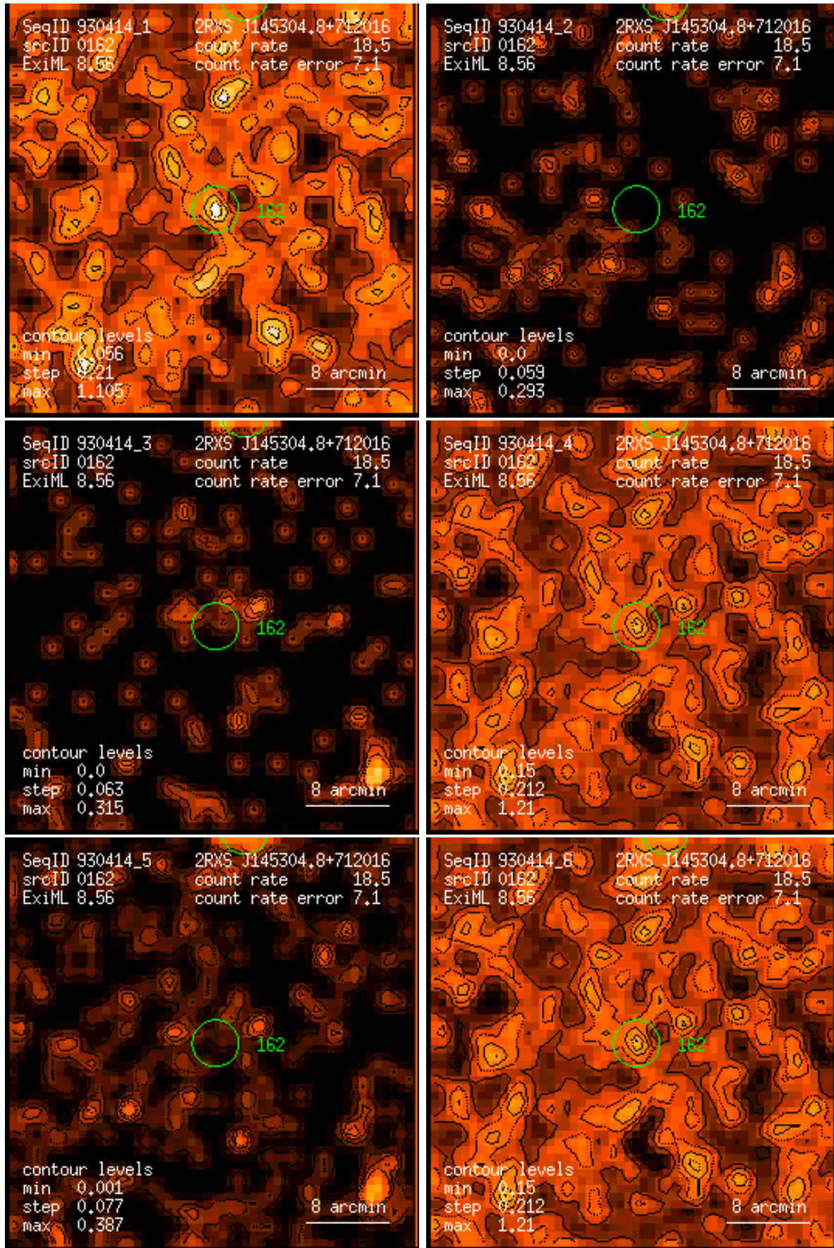
Figure 162: RASS 930414: detection 0162: band rate images, Gaussian filter: (1) PSPC channels 11 – 41, (2) 52 – 90, (3) 91 – 201, (4) 11 – 235, (5) 52 – 201, (6) 11 – 201. Broad band rates in counts/ks. Band rate contour levels in counts/ks/arcmin 2 .
