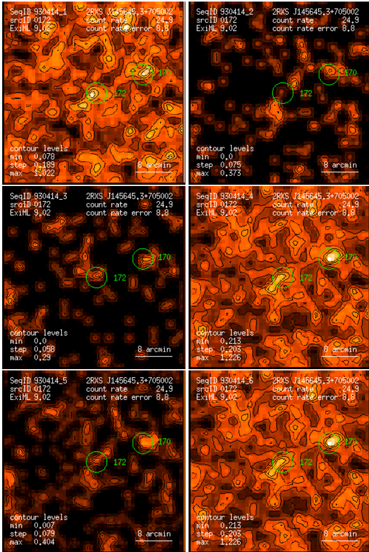
Figure 172: RASS 930414: detection 0172: band rate images, Gaussian filter: (1) PSPC channels 11 – 41, (2) 52 – 90, (3) 91 – 201, (4) 11 – 235, (5) 52 – 201, (6) 11 – 201. Broad band rates in counts/ks. Band rate contour levels in counts/ks/arcmin 2 .
