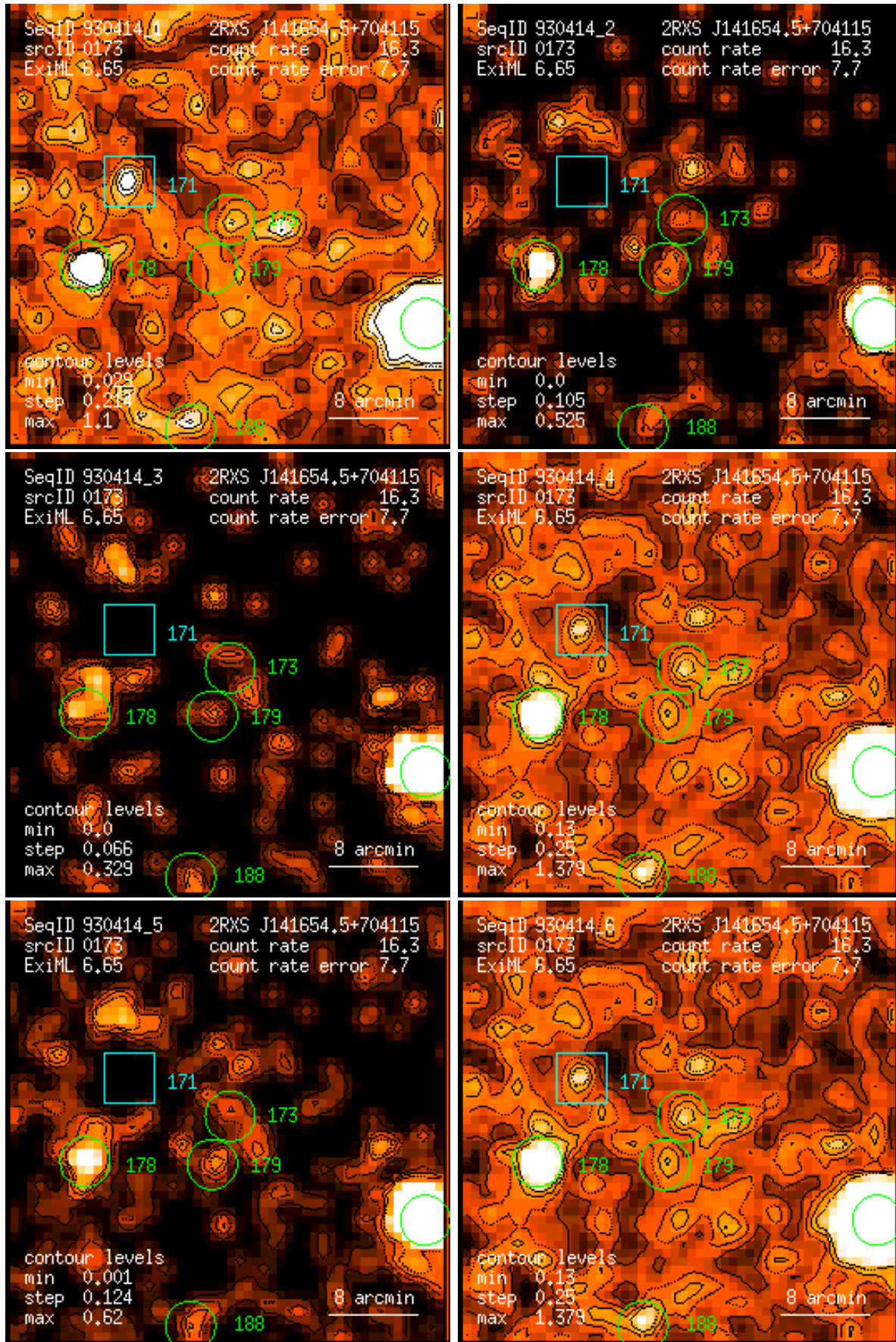
Figure 173: RASS 930414: detection 0173: band rate images, Gaussian filter: (1) PSPC channels 11 – 41, (2) 52 – 90, (3) 91 – 201, (4) 11 – 235, (5) 52 – 201, (6) 11 – 201. Broad band rates in counts/ks. Band rate contour levels in counts/ks/arcmin 2 .
