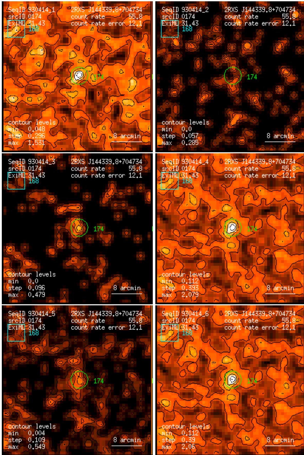
Figure 174: RASS 930414: detection 0174: band rate images, Gaussian filter: (1) PSPC channels 11 – 41, (2) 52 – 90, (3) 91 – 201, (4) 11 – 235, (5) 52 – 201, (6) 11 – 201. Broad band rates in counts/ks. Band rate contour levels in counts/ks/arcmin 2 .
