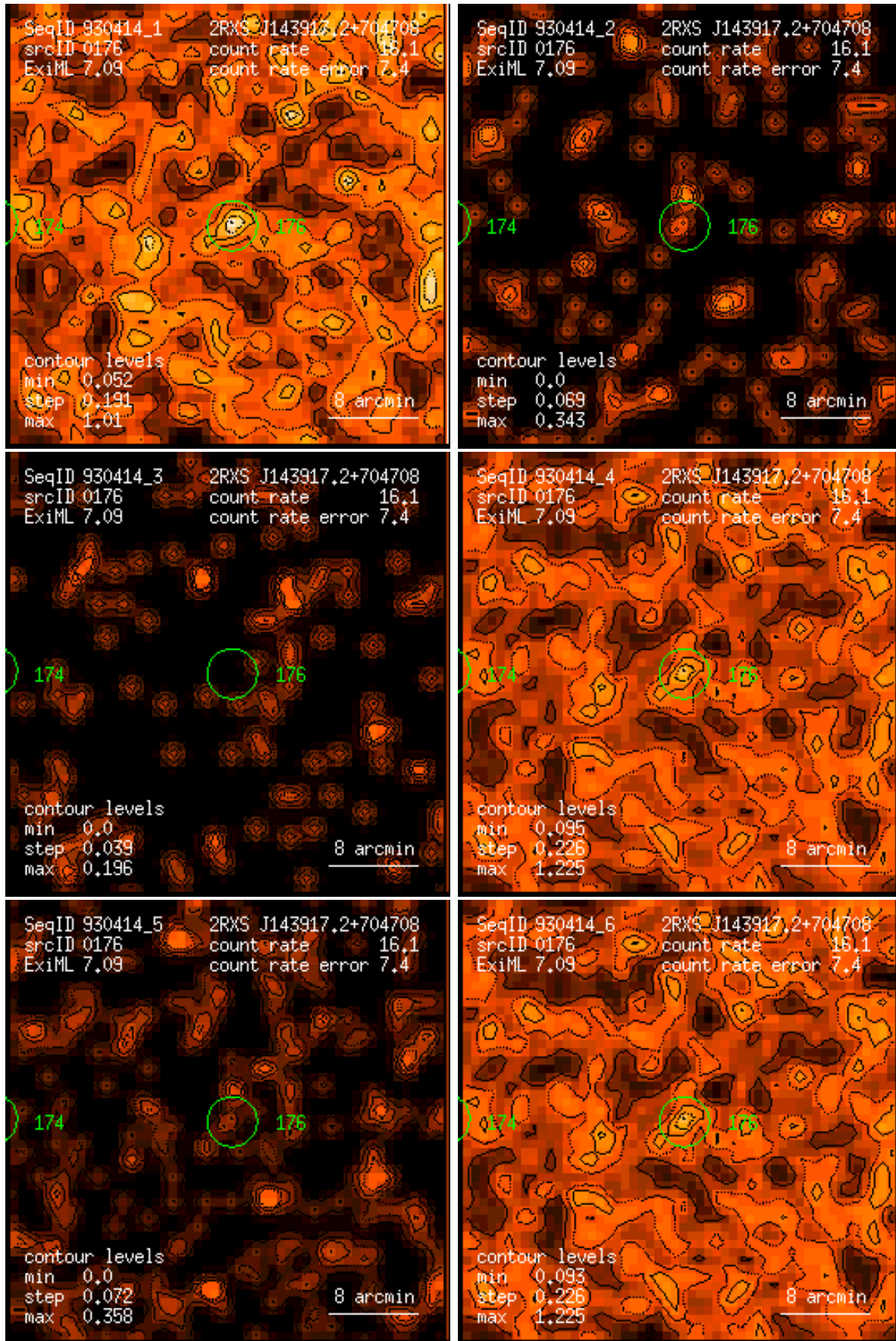
Figure 176: RASS 930414: detection 0176: band rate images, Gaussian filter: (1) PSPC channels 11 – 41, (2) 52 – 90, (3) 91 – 201, (4) 11 – 235, (5) 52 – 201, (6) 11 – 201. Broad band rates in counts/ks. Band rate contour levels in counts/ks/arcmin 2 .
