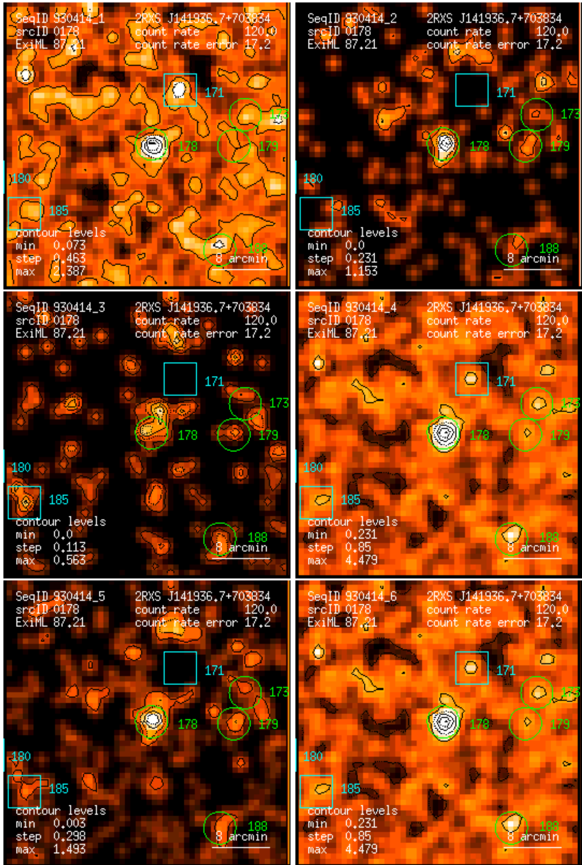
Figure 178: RASS 930414: detection 0178: band rate images, Gaussian filter: (1) PSPC channels 11 – 41, (2) 52 – 90, (3) 91 – 201, (4) 11 – 235, (5) 52 – 201, (6) 11 – 201. Broad band rates in counts/ks. Band rate contour levels in counts/ks/arcmin 2 .
