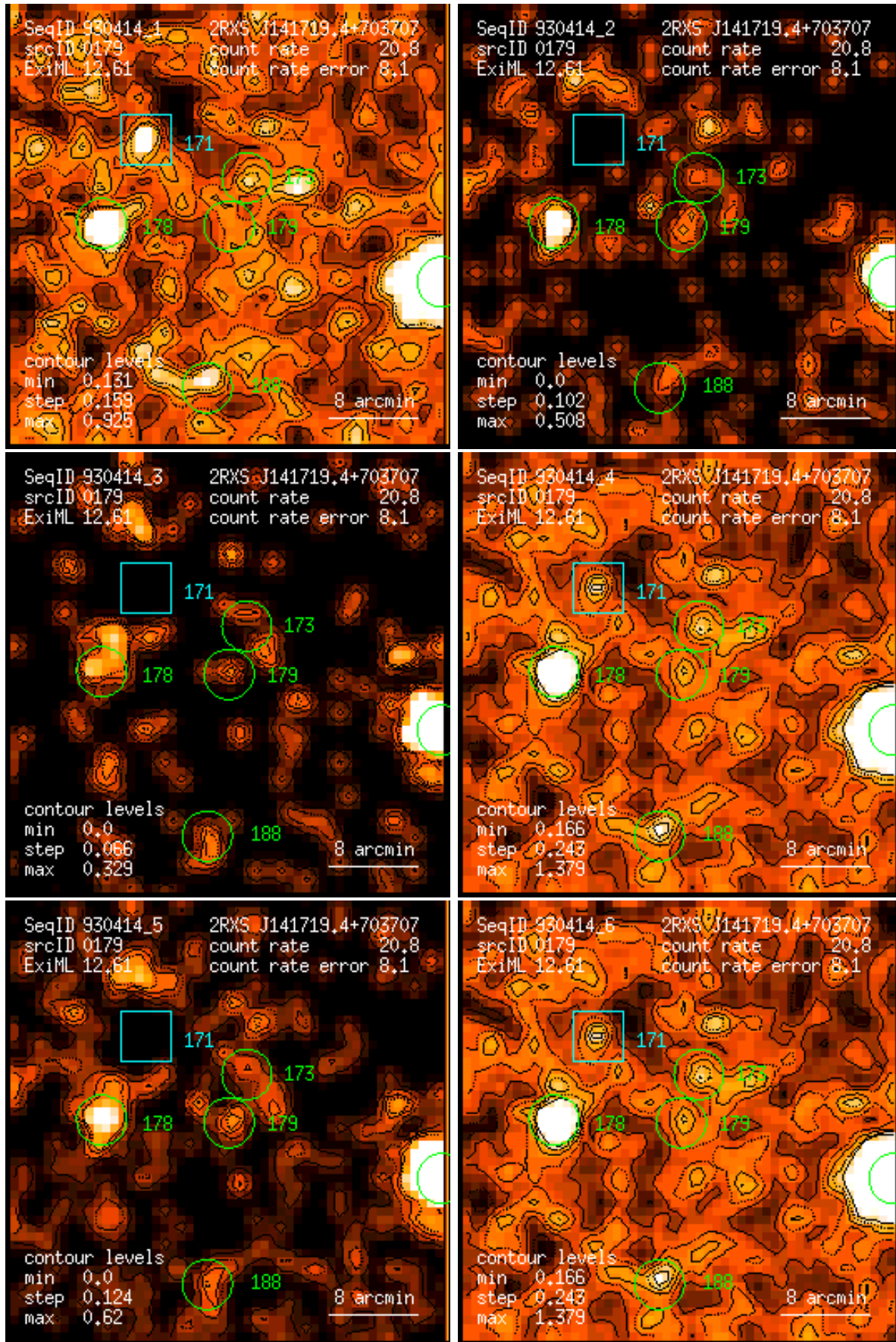
Figure 179: RASS 930414: detection 0179: band rate images, Gaussian filter: (1) PSPC channels 11 – 41, (2) 52 – 90, (3) 91 – 201, (4) 11 – 235, (5) 52 – 201, (6) 11 – 201. Broad band rates in counts/ks. Band rate contour levels in counts/ks/arcmin 2 .
