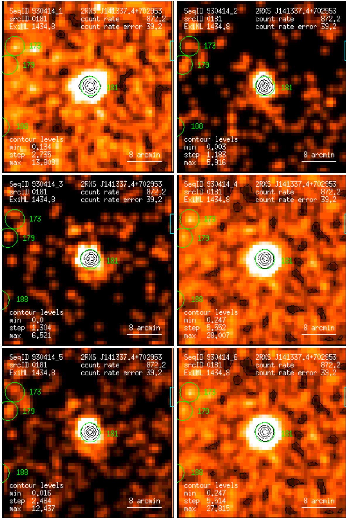
Figure 181: RASS 930414: detection 0181: band rate images, Gaussian filter: (1) PSPC channels 11 – 41, (2) 52 – 90, (3) 91 – 201, (4) 11 – 235, (5) 52 – 201, (6) 11 – 201. Broad band rates in counts/ks. Band rate contour levels in counts/ks/arcmin 2 .
