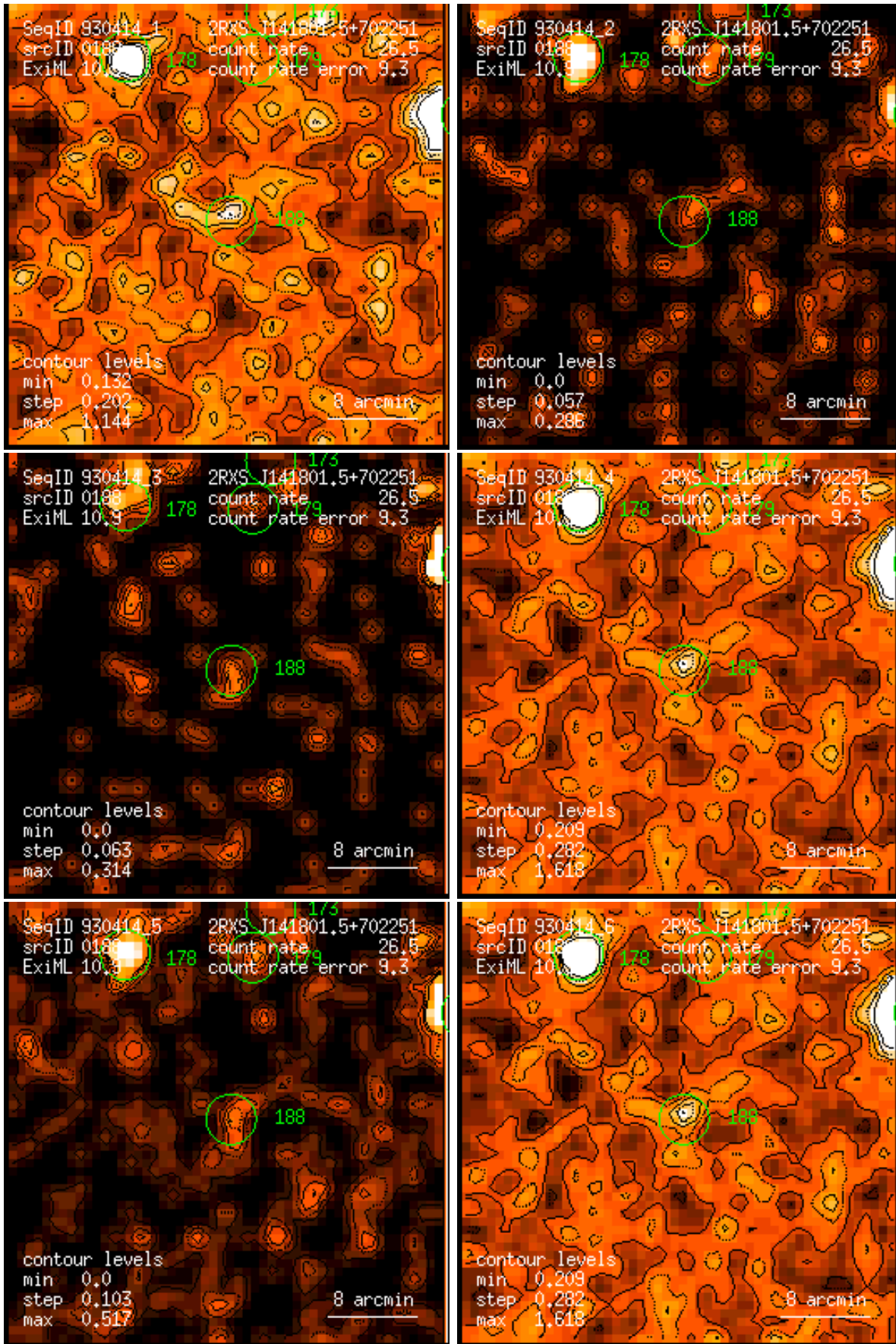
Figure 188: RASS 930414: detection 0188: band rate images, Gaussian filter: (1) PSPC channels 11 – 41, (2) 52 – 90, (3) 91 – 201, (4) 11 – 235, (5) 52 – 201, (6) 11 – 201. Broad band rates in counts/ks. Band rate contour levels in counts/ks/arcmin 2 .
