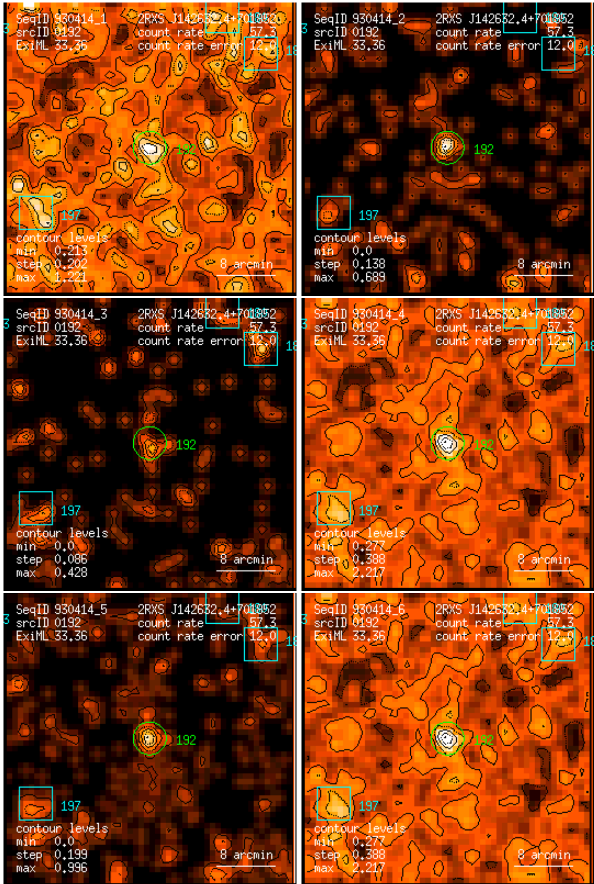
Figure 192: RASS 930414: detection 0192: band rate images, Gaussian filter: (1) PSPC channels 11 – 41, (2) 52 – 90, (3) 91 – 201, (4) 11 – 235, (5) 52 – 201, (6) 11 – 201. Broad band rates in counts/ks. Band rate contour levels in counts/ks/arcmin 2 .
