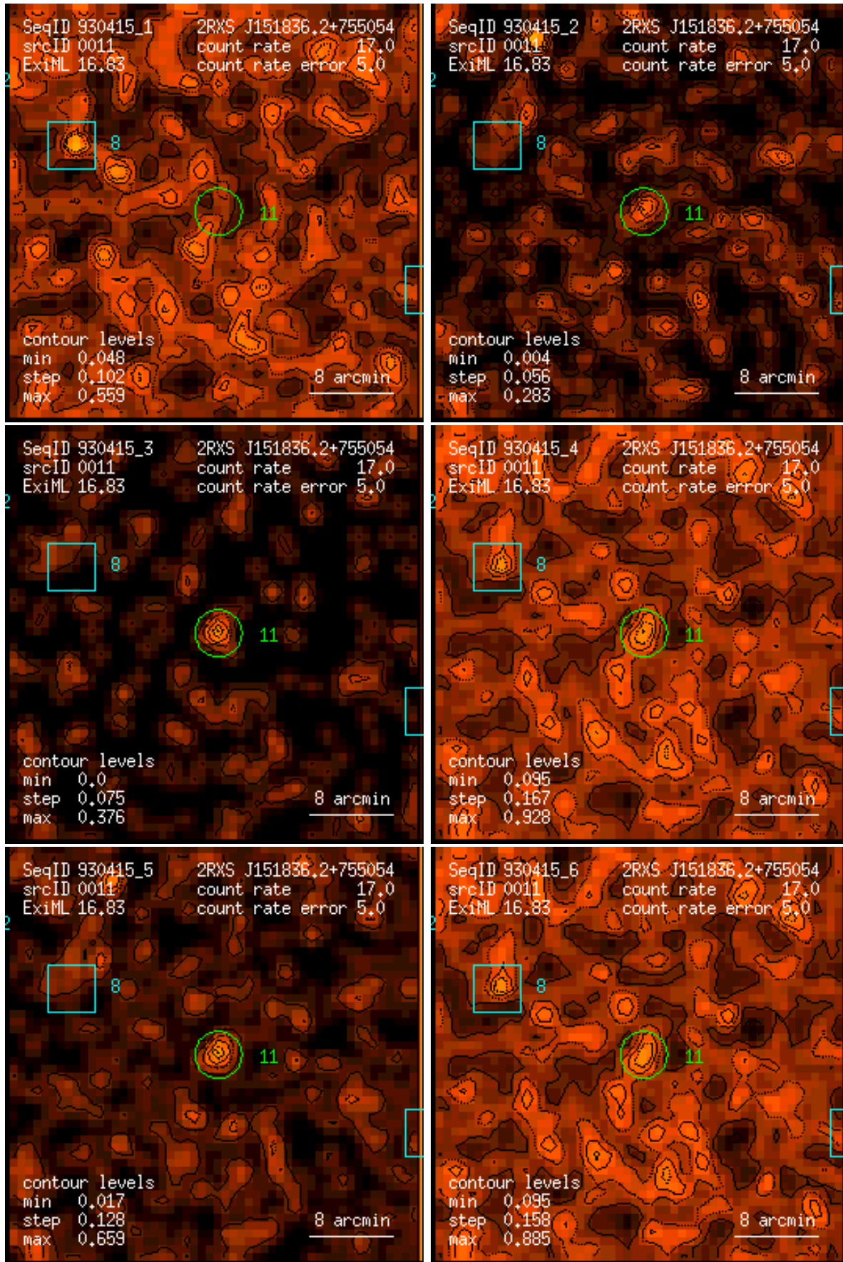
Figure 11: RASS 930415: detection 0011: band rate images, Gaussian filter: (1) PSPC channels 11 – 41, (2) 52 – 90, (3) 91 – 201, (4) 11 – 235, (5) 52 – 201, (6) 11 – 201. Broad band rates in counts/ks. Band rate contour levels in counts/ks/arcmin 2 .
