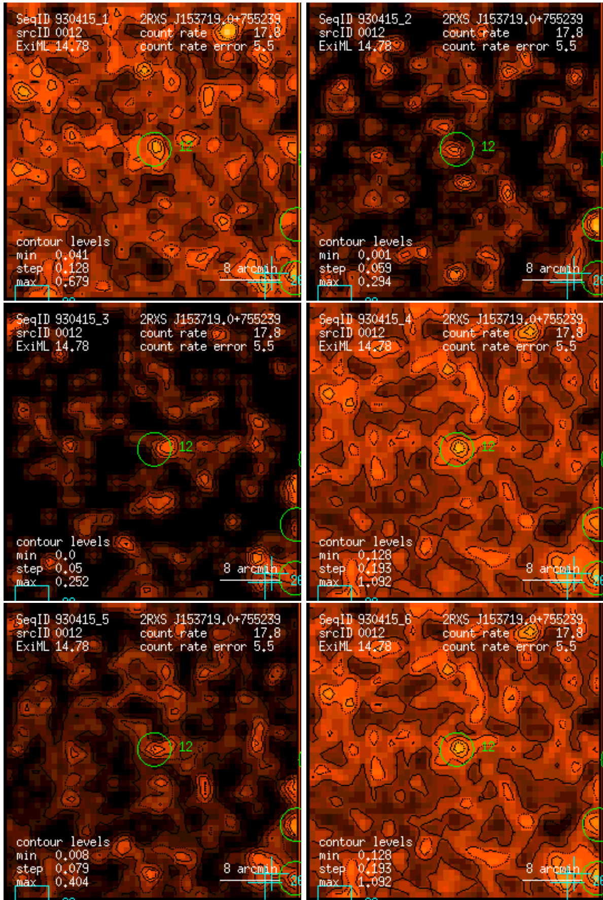
Figure 12: RASS 930415: detection 0012: band rate images, Gaussian filter: (1) PSPC channels 11 – 41, (2) 52 – 90, (3) 91 – 201, (4) 11 – 235, (5) 52 – 201, (6) 11 – 201. Broad band rates in counts/ks. Band rate contour levels in counts/ks/arcmin 2 .
