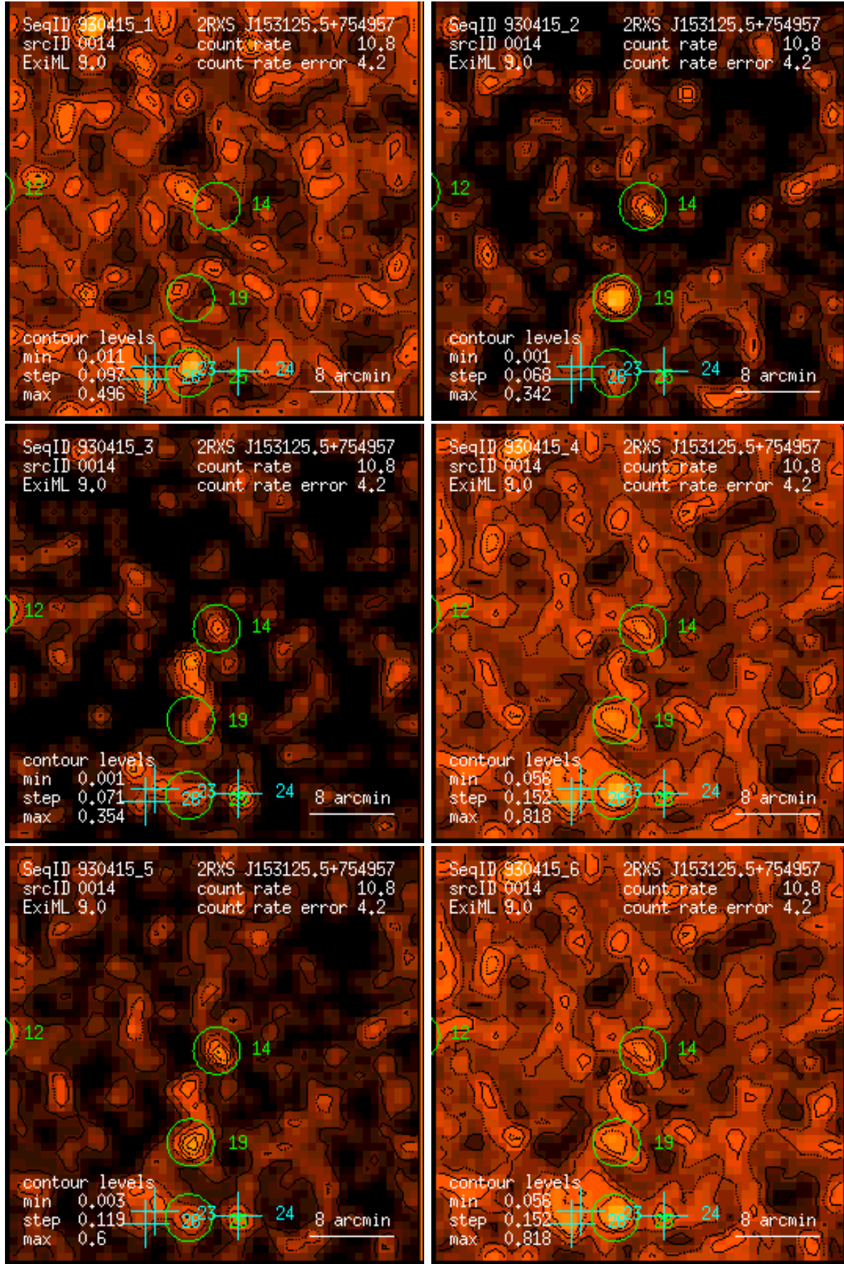
Figure 14: RASS 930415: detection 0014: band rate images, Gaussian filter: (1) PSPC channels 11 – 41, (2) 52 – 90, (3) 91 – 201, (4) 11 – 235, (5) 52 – 201, (6) 11 – 201. Broad band rates in counts/ks. Band rate contour levels in counts/ks/arcmin 2 .
